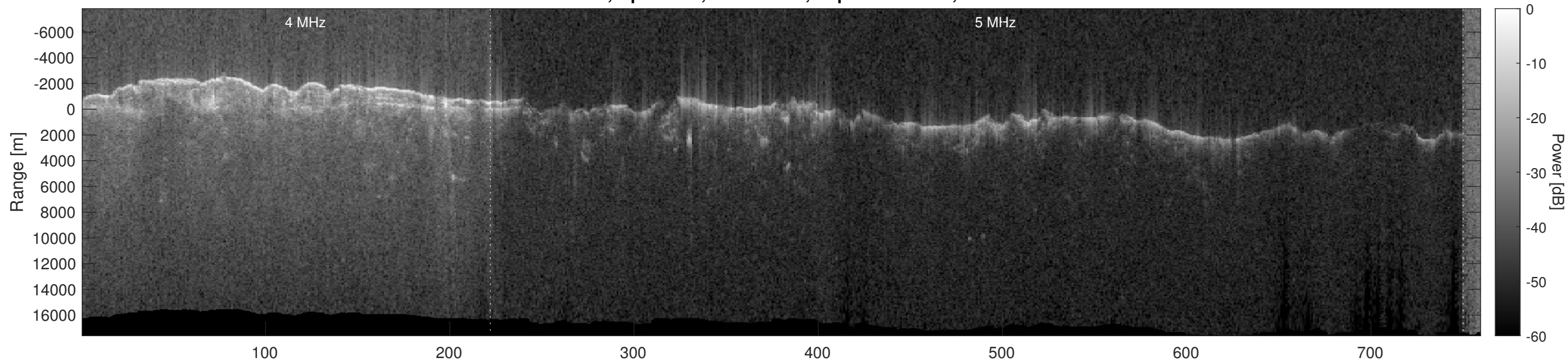
Orbit 14756, Optimized, No Window, Depth-Corrected, Channel 2
