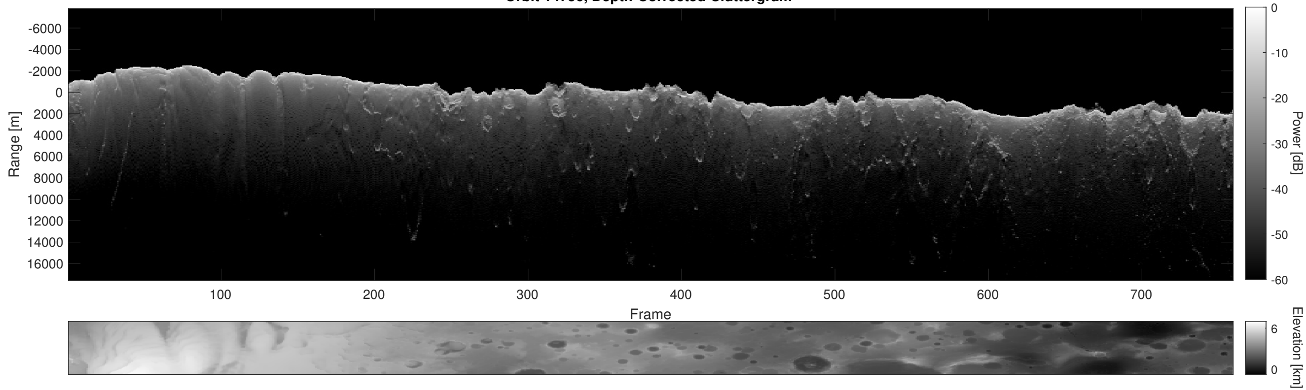
Orbit 14756, Depth-Corrected Cluttergram
