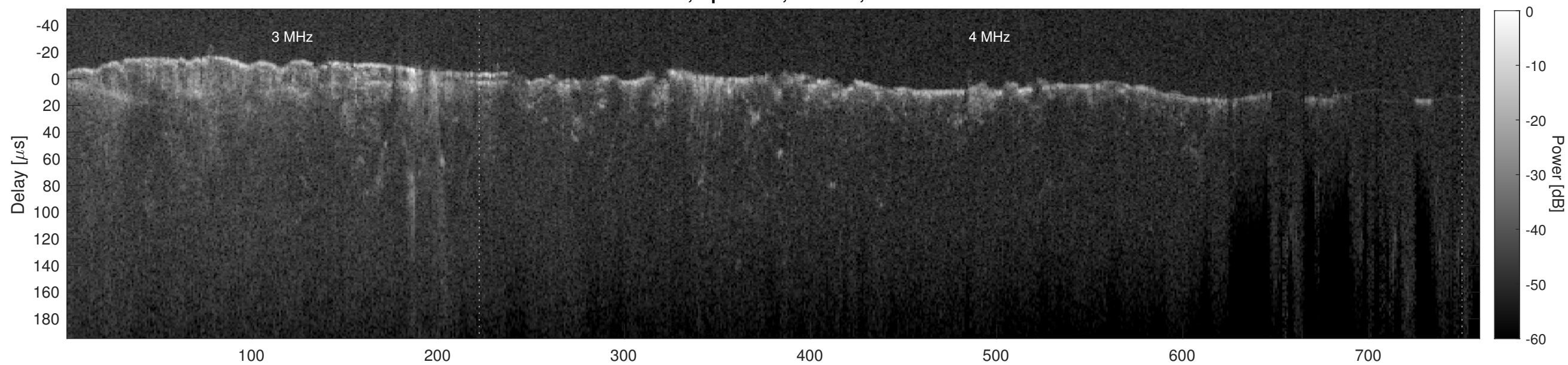
Orbit 14756, Cluttergram
