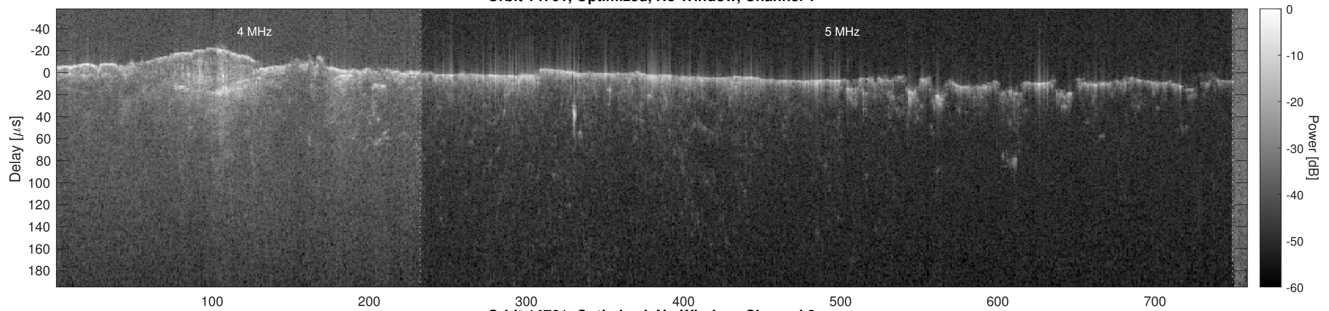
Orbit 14761, Optimized, No Window, Channel 2
