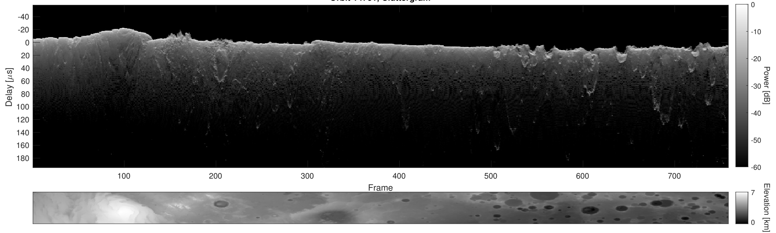
Orbit 14761, Cluttergram
