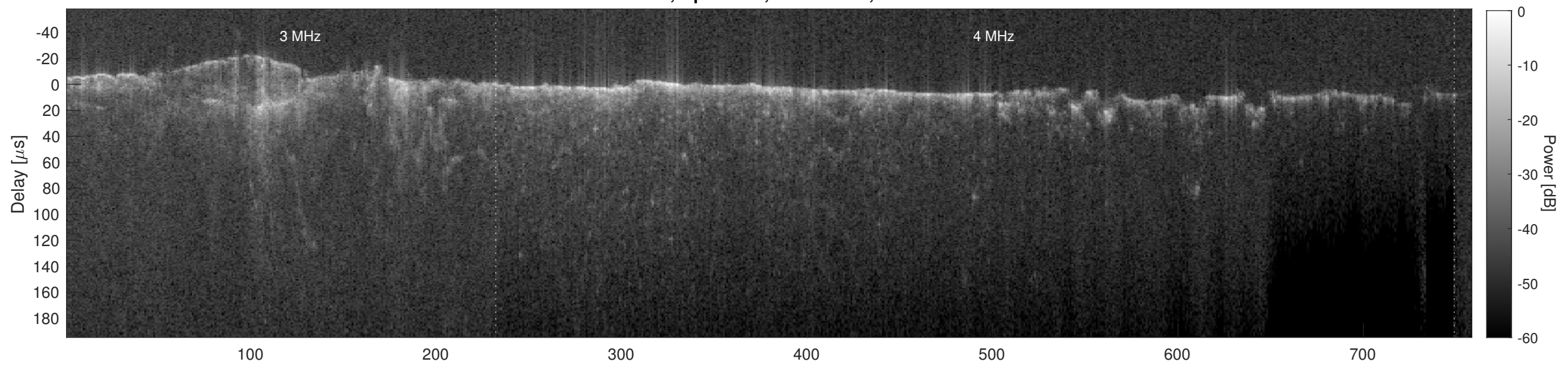
Orbit 14761, Cluttergram
