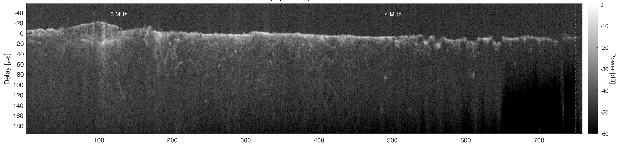
Orbit 14761, Cluttergram
