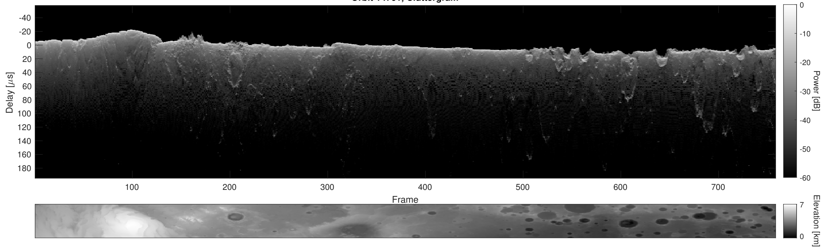
Orbit 14761, Cluttergram
