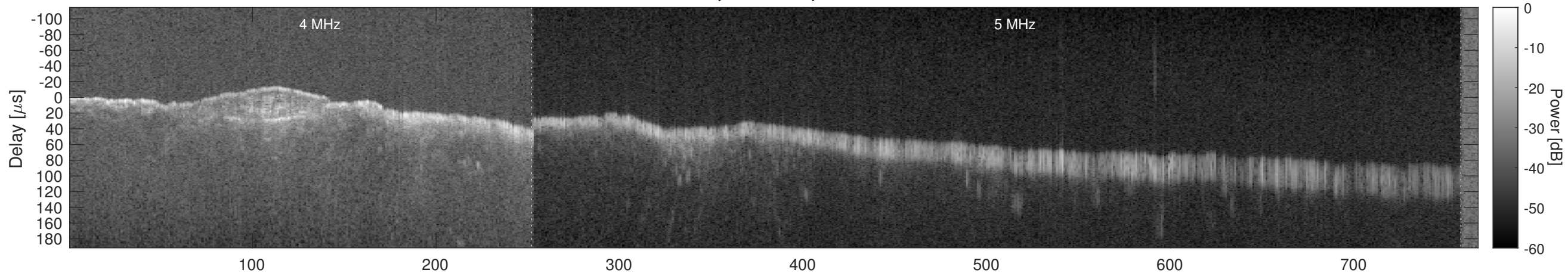
Orbit 14768, Window, Channel 1, Chapman
