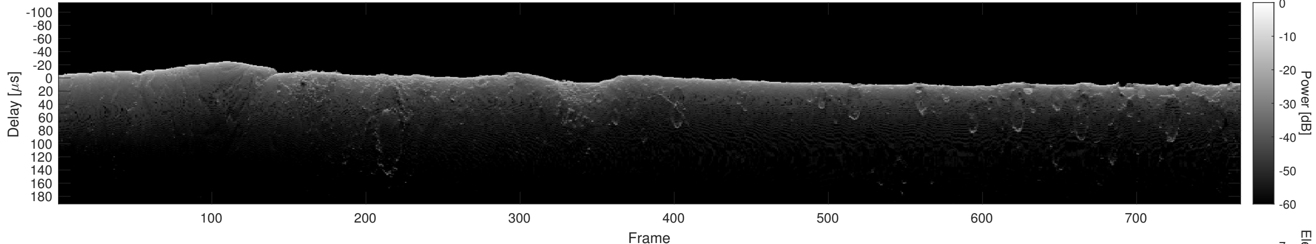
Orbit 14768, Cluttergram
