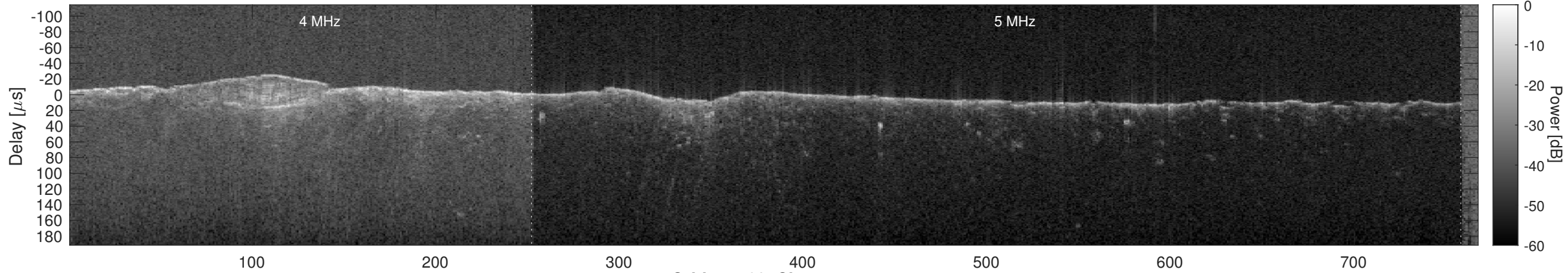
Orbit 14768, Cluttergram
