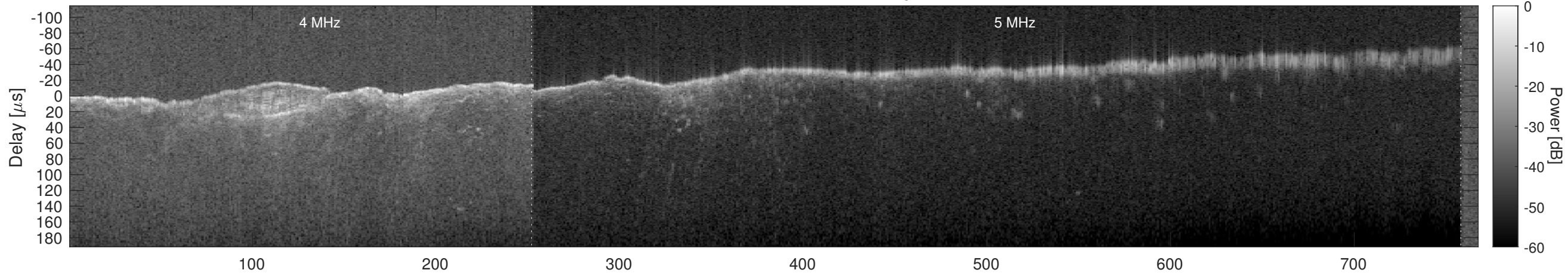
Orbit 14768, Window, Channel 1, Optimized
