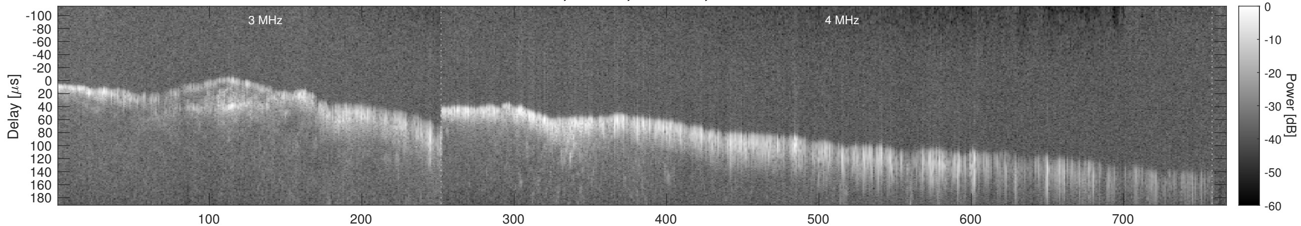
Orbit 14768, Window, Channel 2, Chapman
