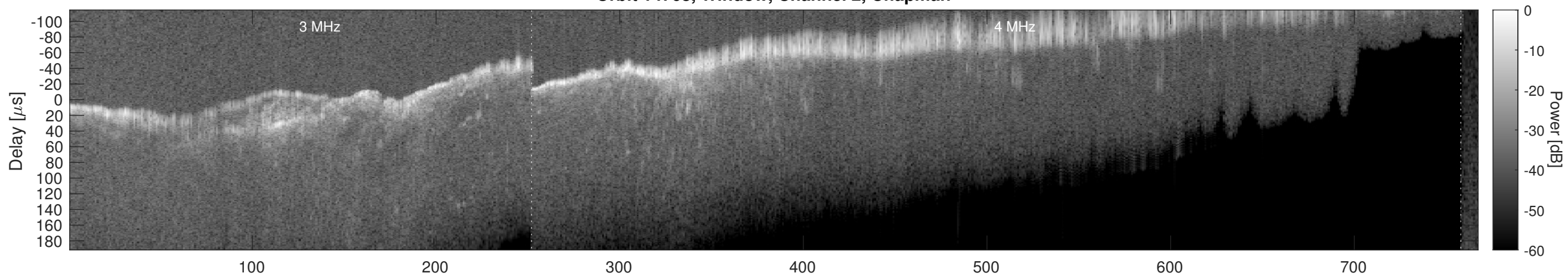
Orbit 14768, Window, Channel 2, Optimized
