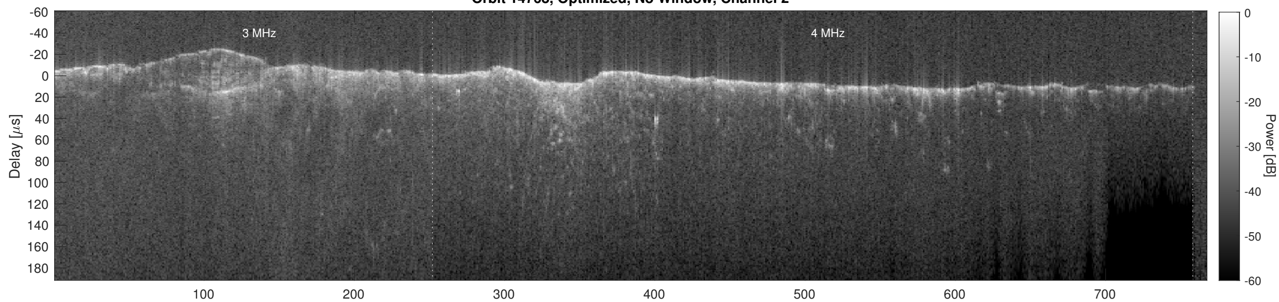
Orbit 14768, Cluttergram
