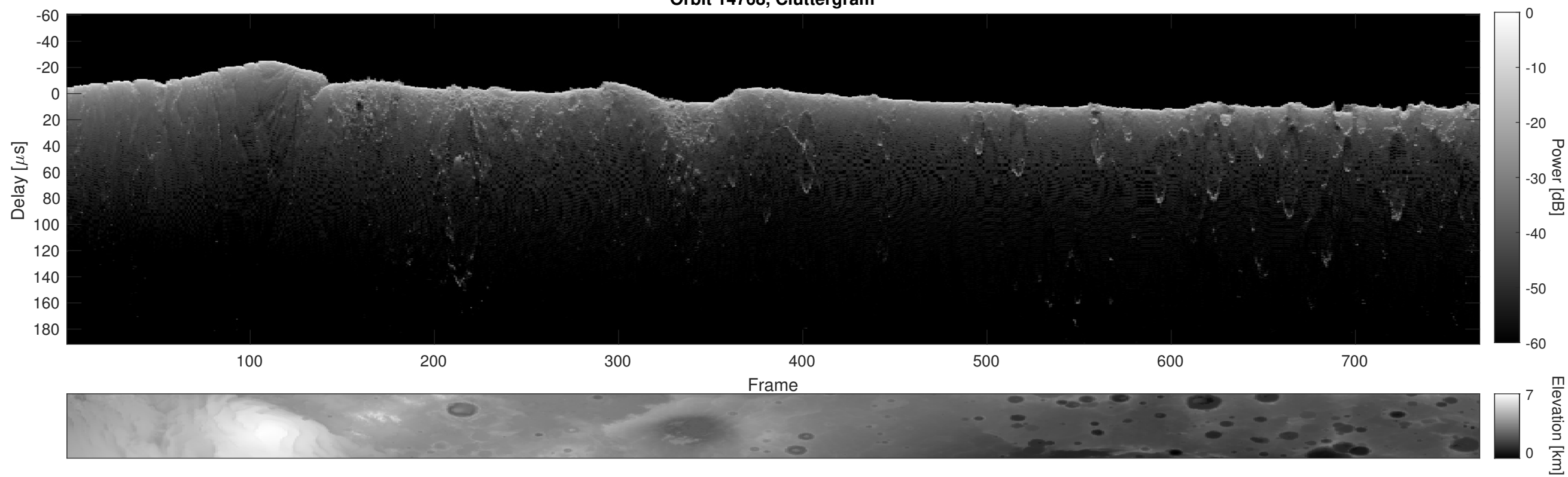
Orbit 14768, Cluttergram
