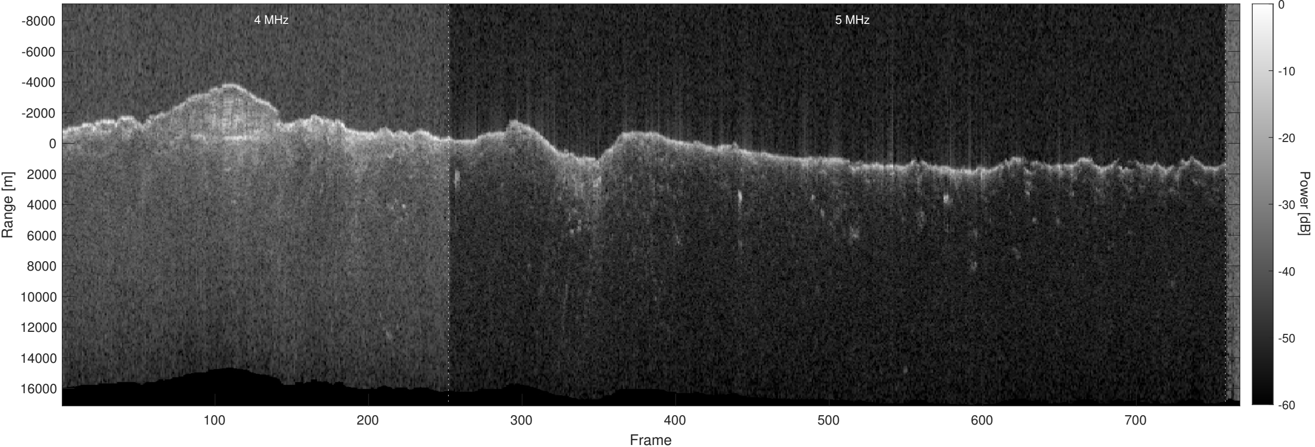
Orbit 14768, Optimized, Window, Depth-Corrected, Channel 2
