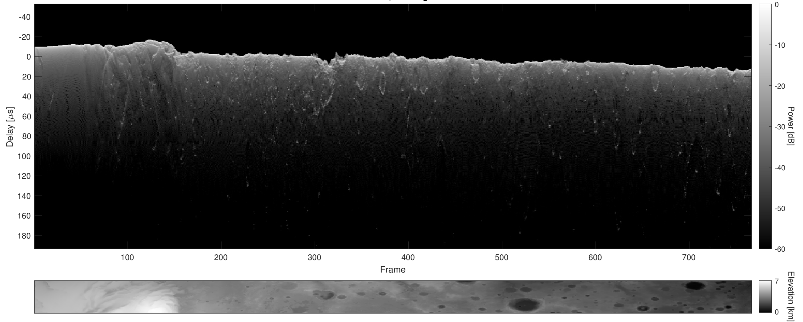
Orbit 14772, Cluttergram
