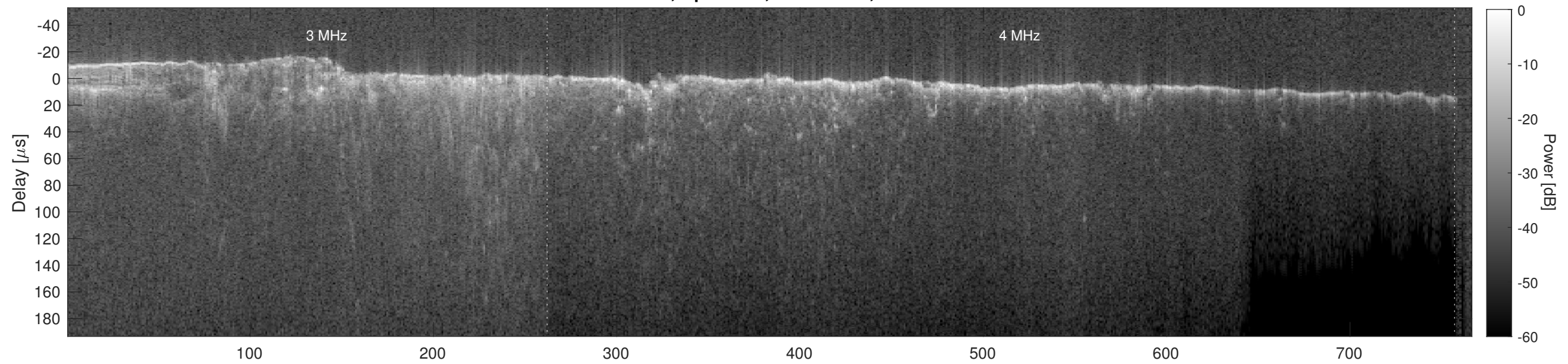
Orbit 14772, Cluttergram
