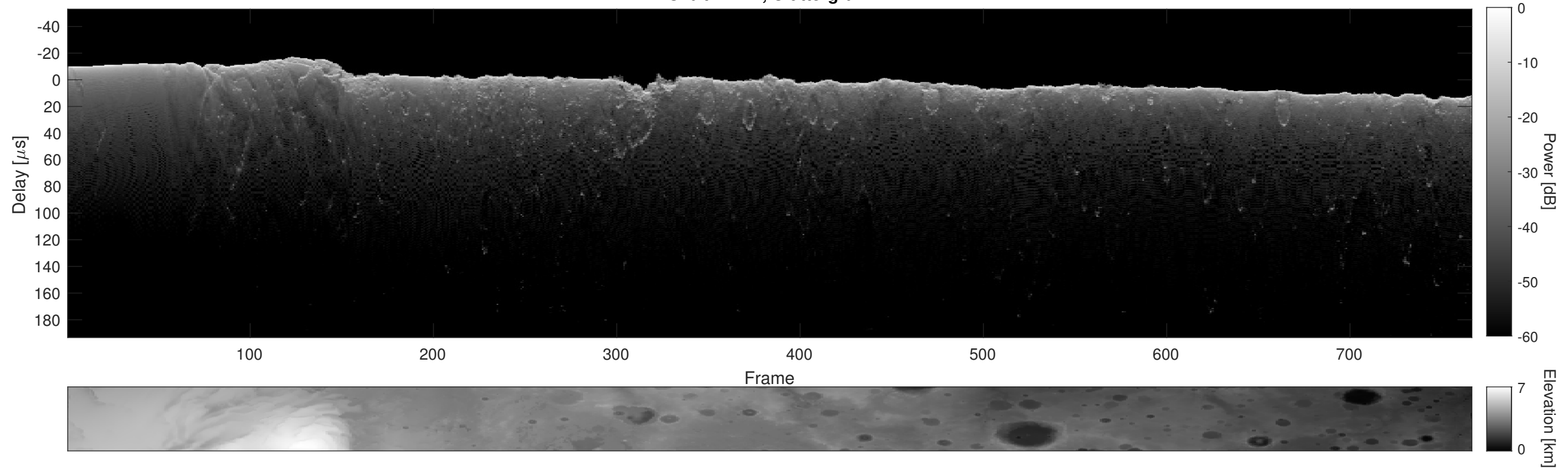
Orbit 14772, Cluttergram
