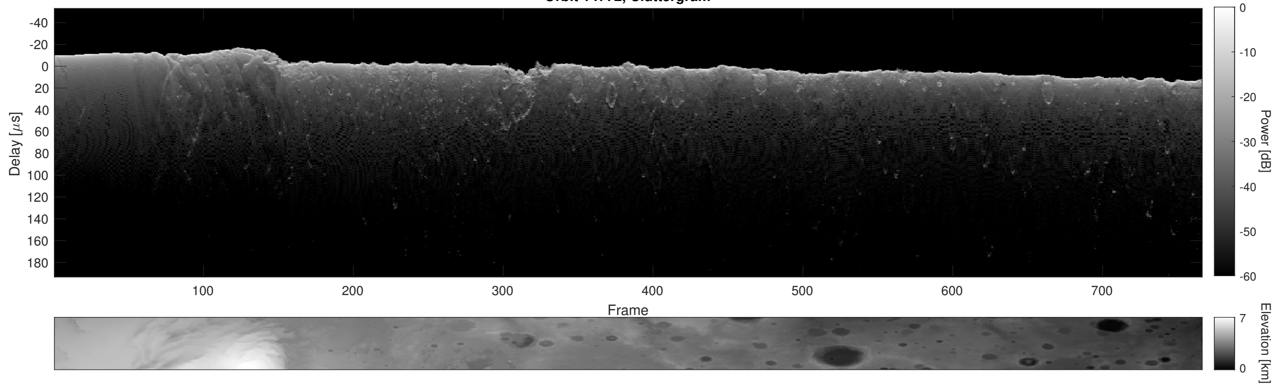
Orbit 14772, Cluttergram
