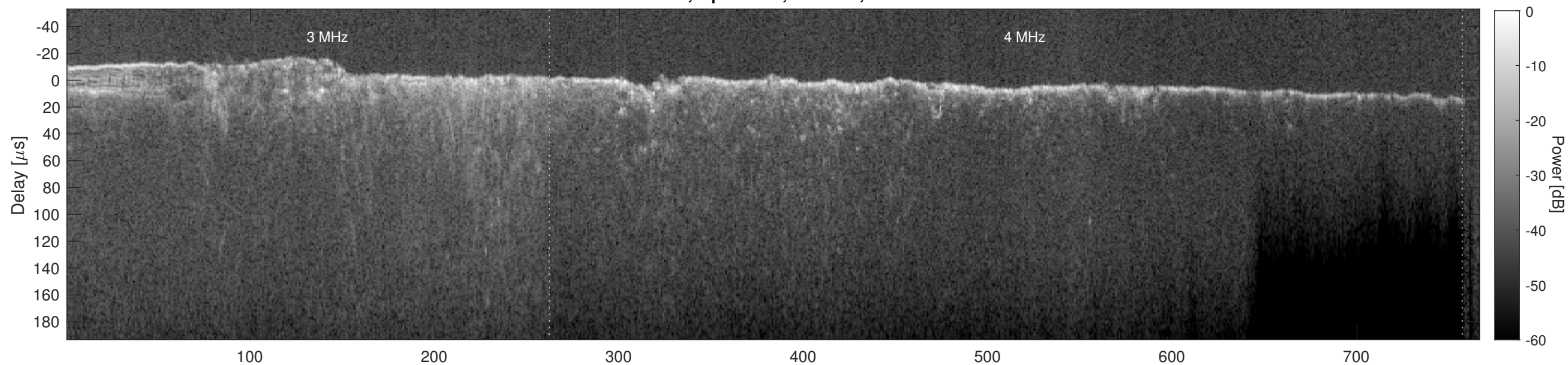
Orbit 14772, Cluttergram
