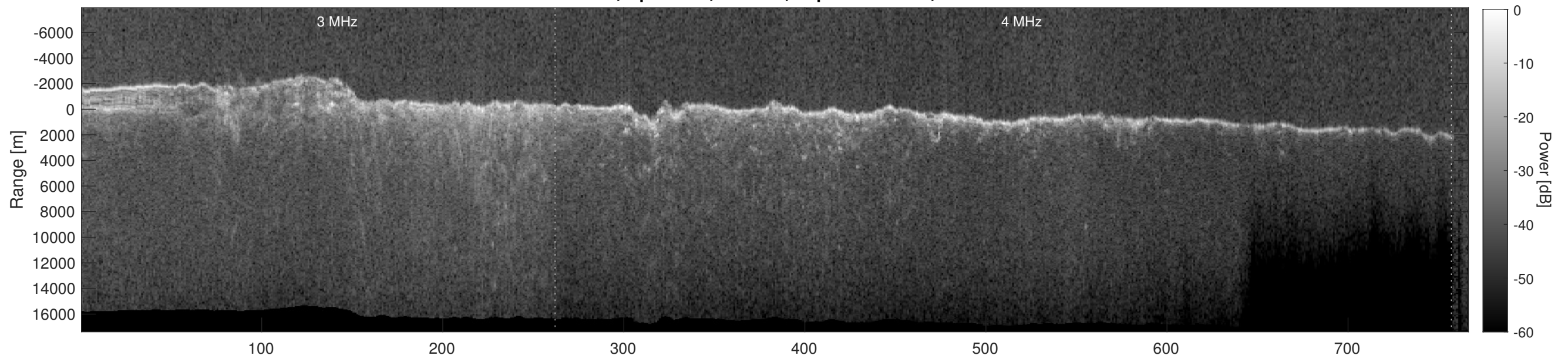
Orbit 14772, Depth-Corrected Cluttergram
