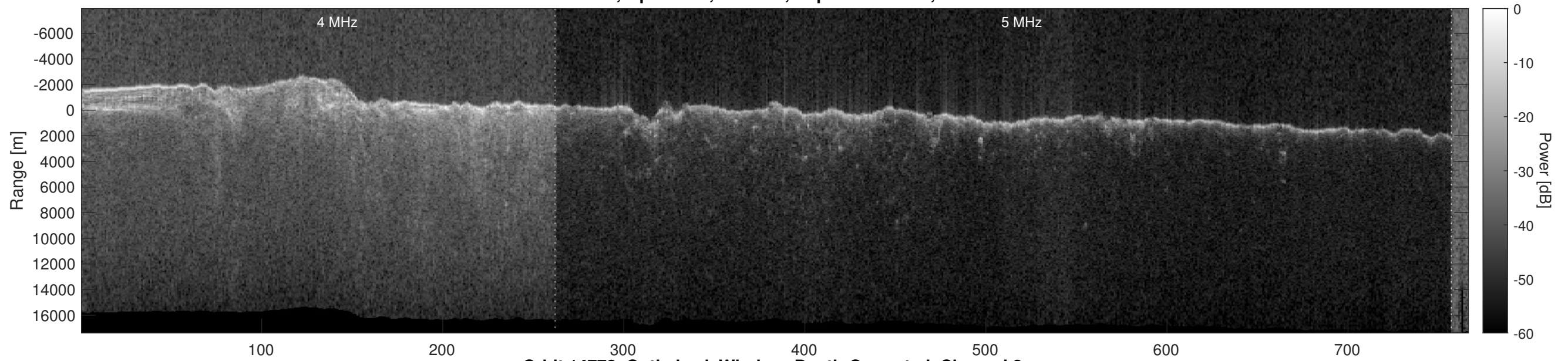
Orbit 14772, Optimized, Window, Depth-Corrected, Channel 2
