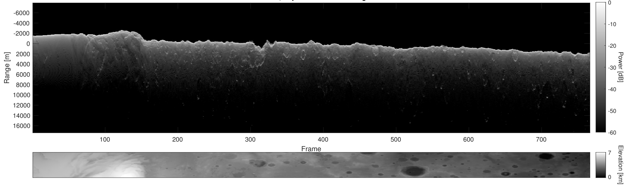
Orbit 14772, Depth-Corrected Cluttergram
