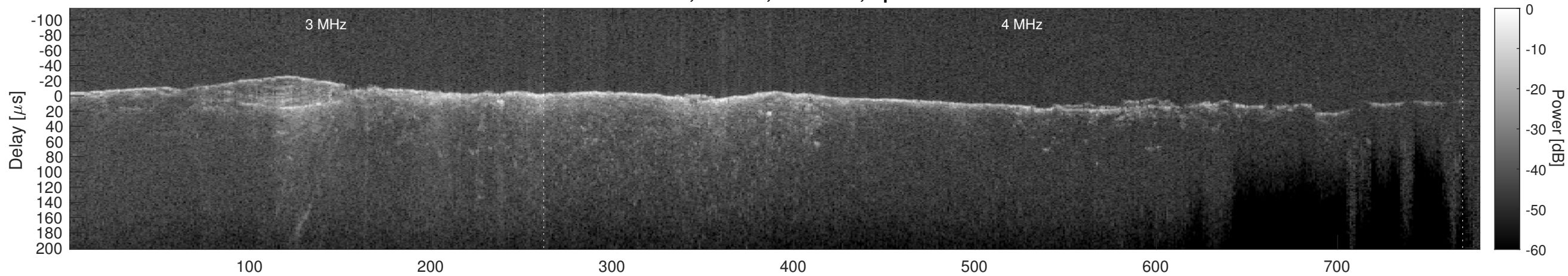
Orbit 14775, Cluttergram
