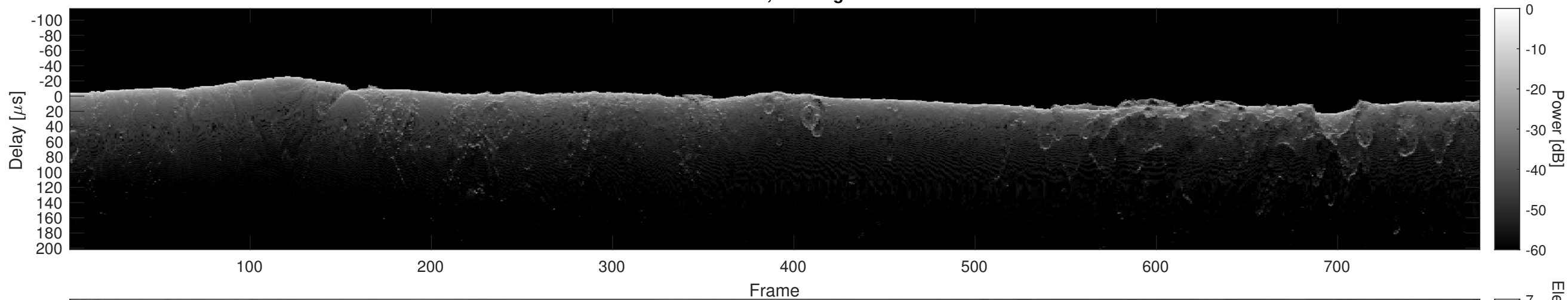
Orbit 14775, Cluttergram
