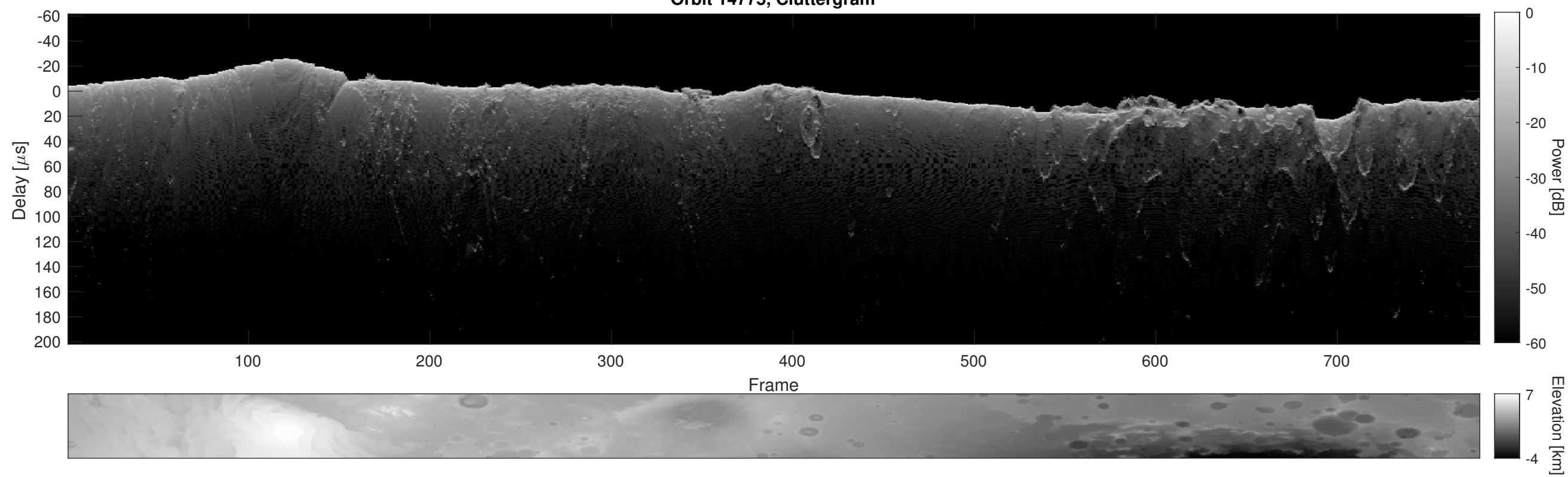
Orbit 14775, Cluttergram
