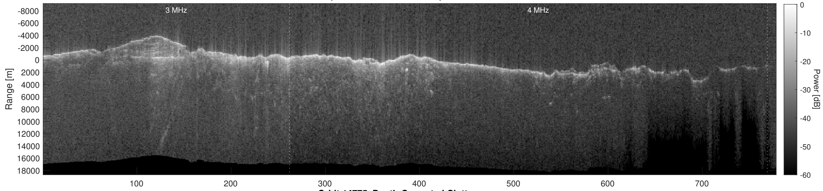
Orbit 14775, Depth-Corrected Cluttergram
