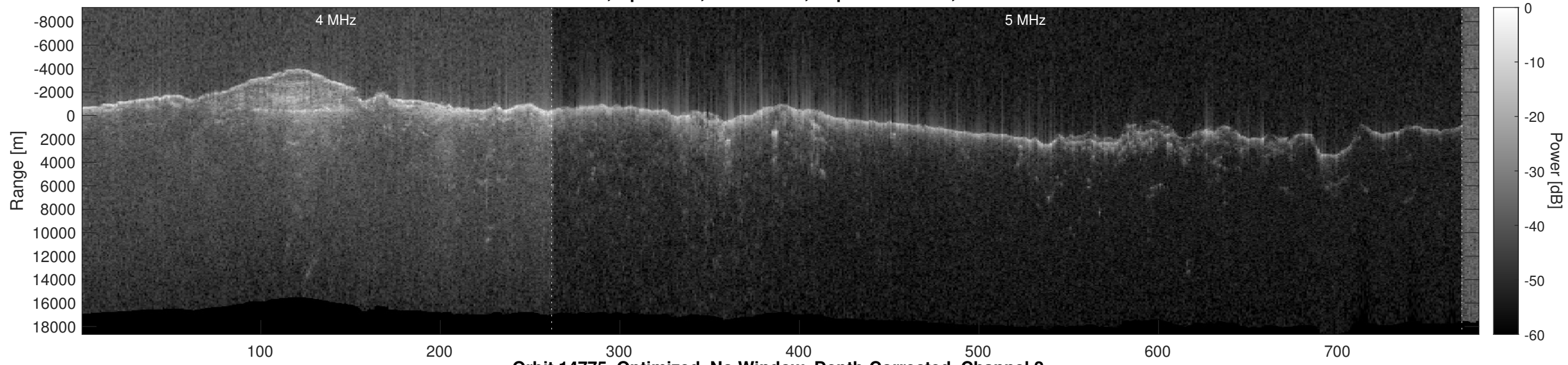
Orbit 14775, Optimized, No Window, Depth-Corrected, Channel 2
