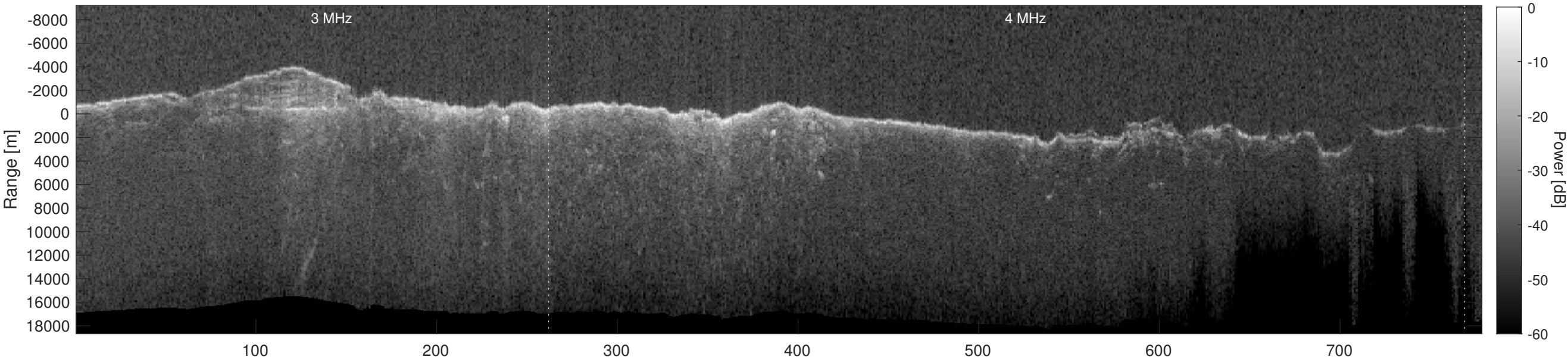
Orbit 14775, Depth-Corrected Cluttergram
