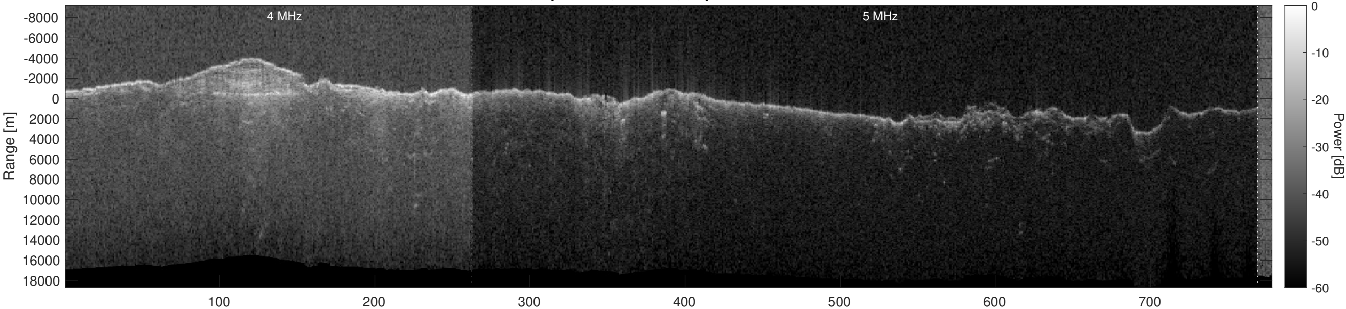
Orbit 14775, Optimized, Window, Depth-Corrected, Channel 2
