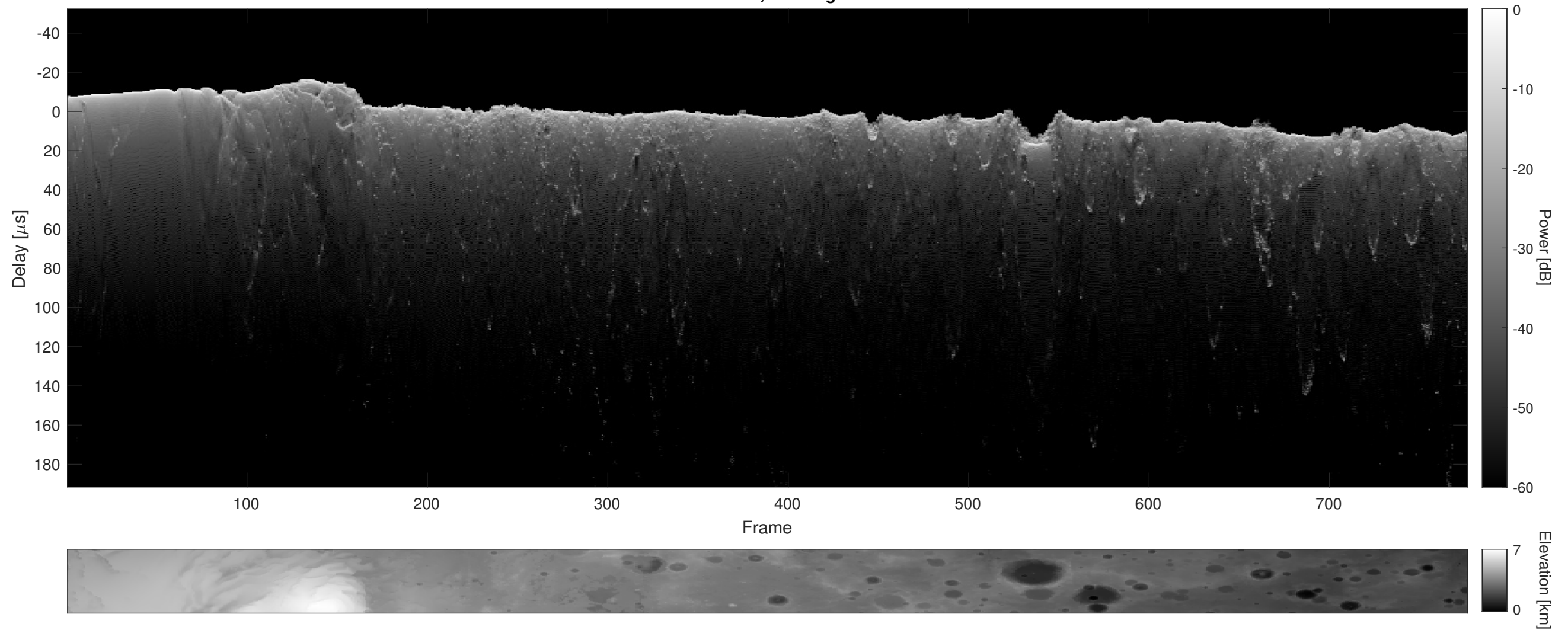
Orbit 14779, Cluttergram
