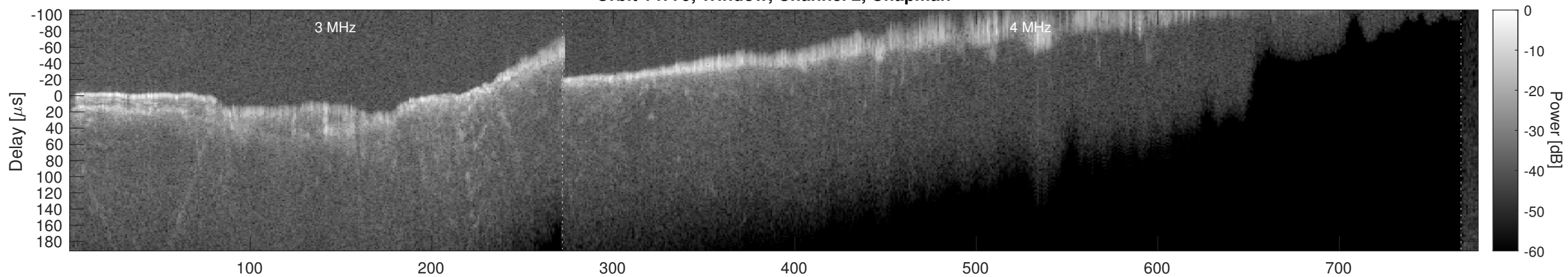
Orbit 14779, Window, Channel 2, Optimized
