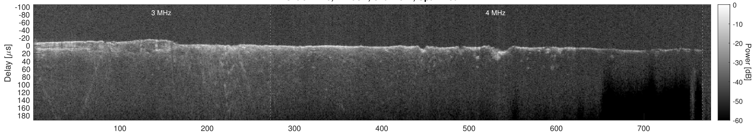
Orbit 14779, Cluttergram
