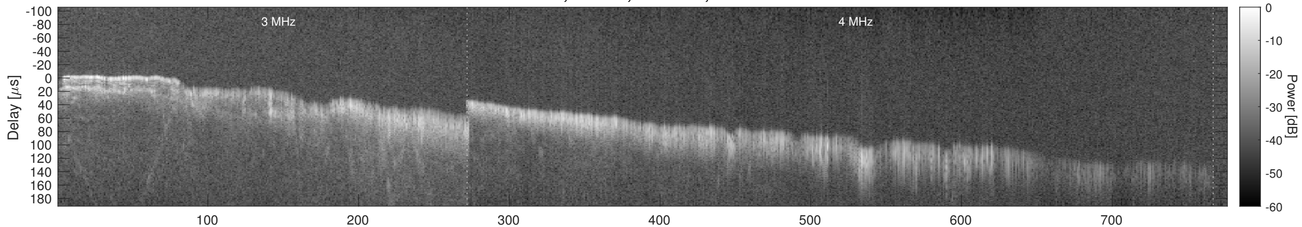
Orbit 14779, Window, Channel 2, Chapman
