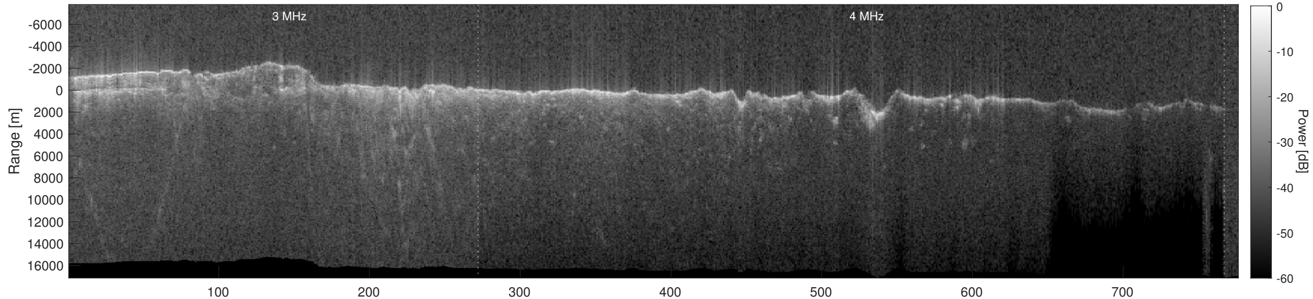
Orbit 14779, Depth-Corrected Cluttergram
