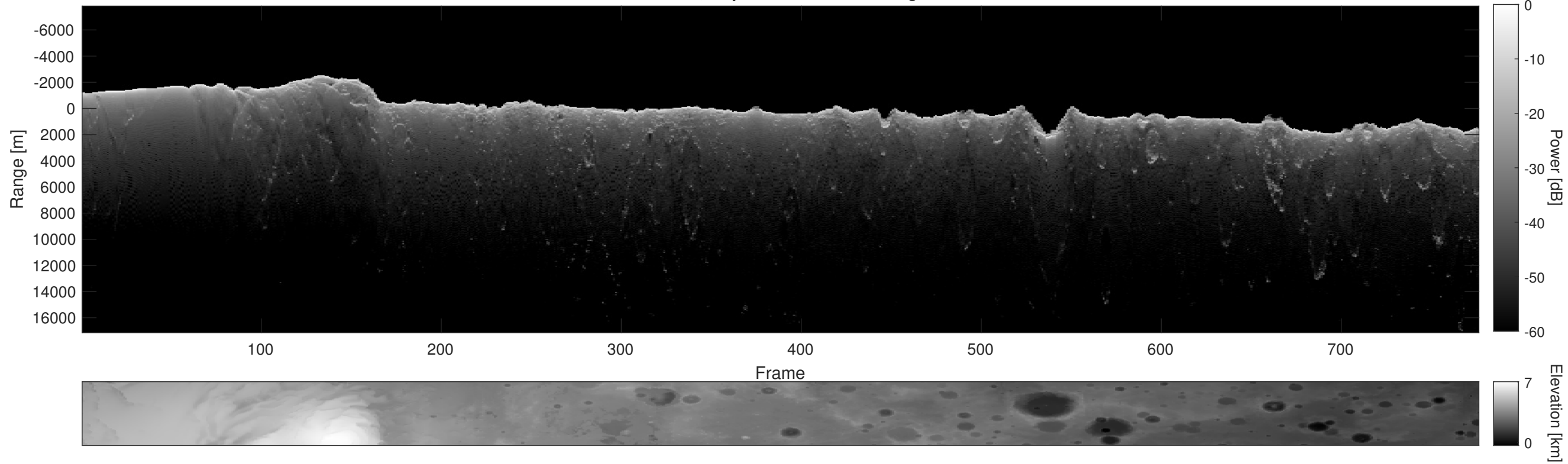
Orbit 14779, Depth-Corrected Cluttergram
