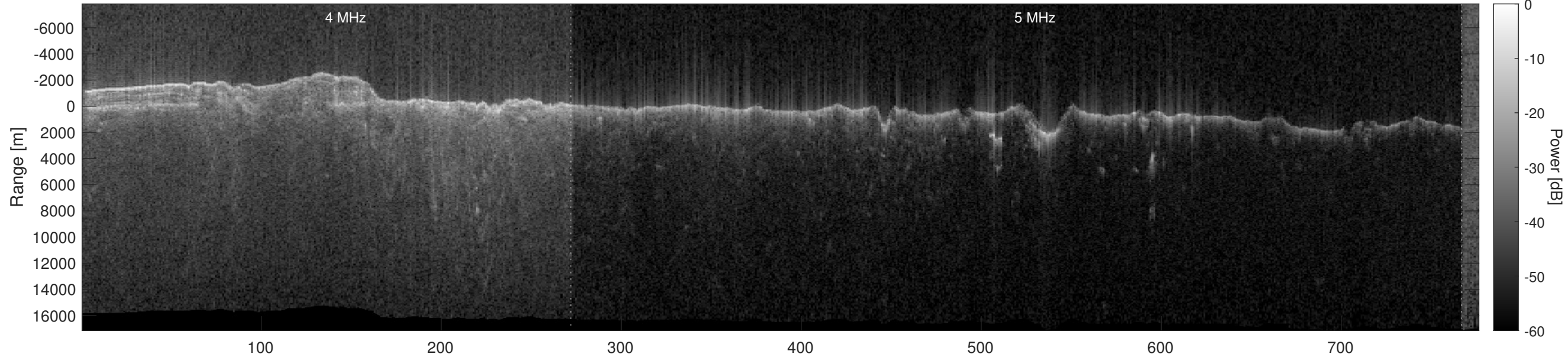
Orbit 14779, Optimized, No Window, Depth-Corrected, Channel 2
