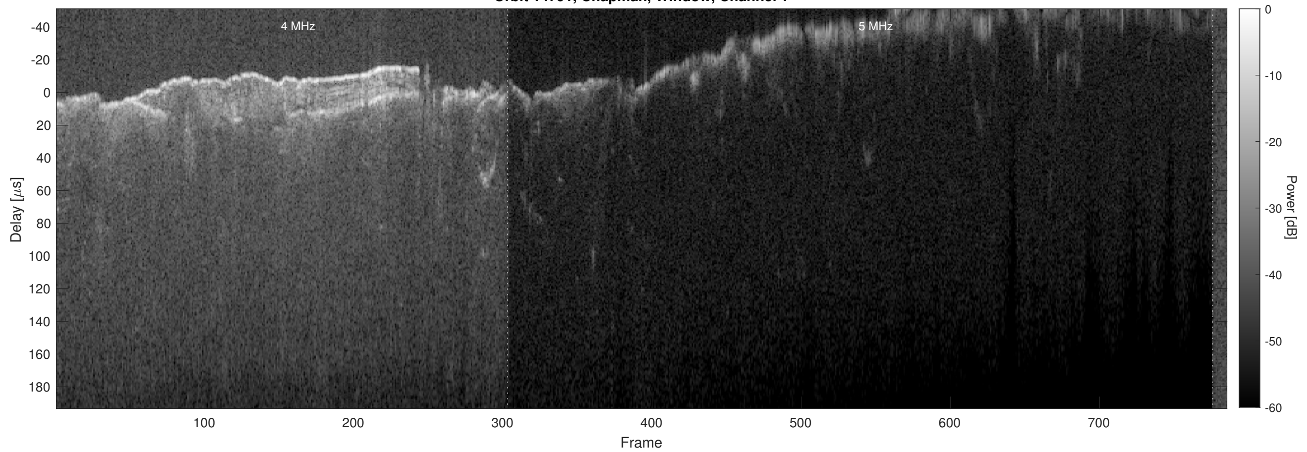
Orbit 14791, Chapman, Window, Channel 2
