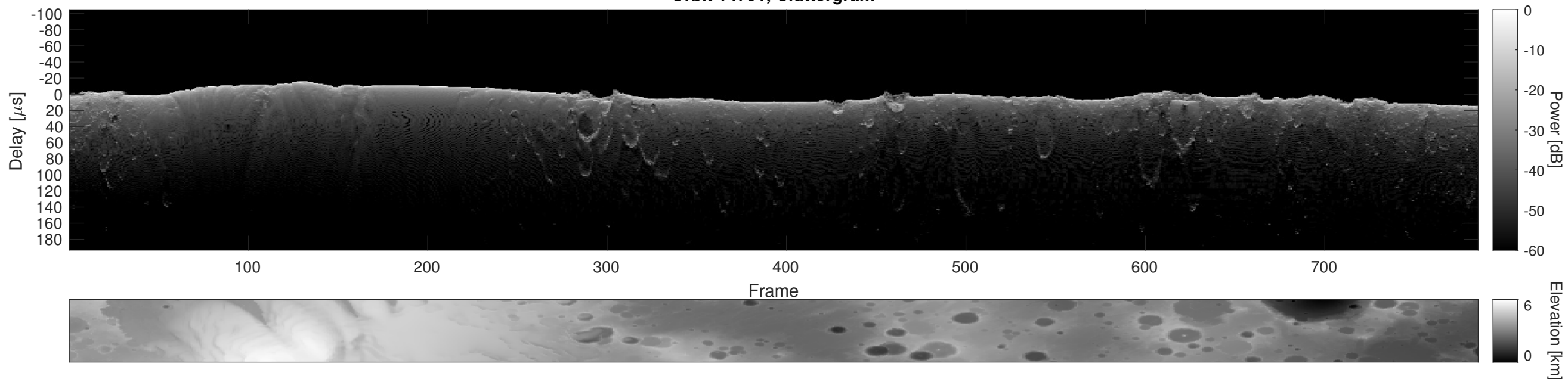
Orbit 14791, Cluttergram
