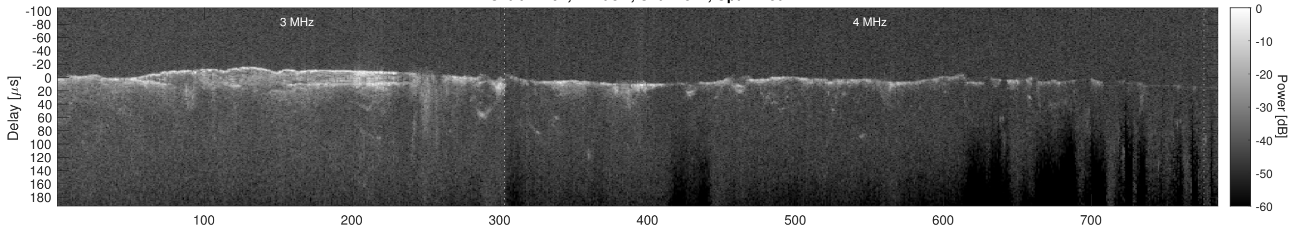
Orbit 14791, Cluttergram
