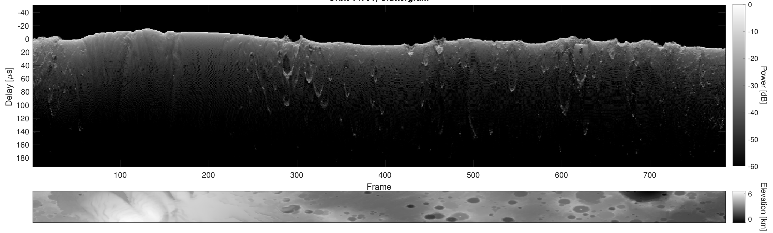
Orbit 14791, Cluttergram
