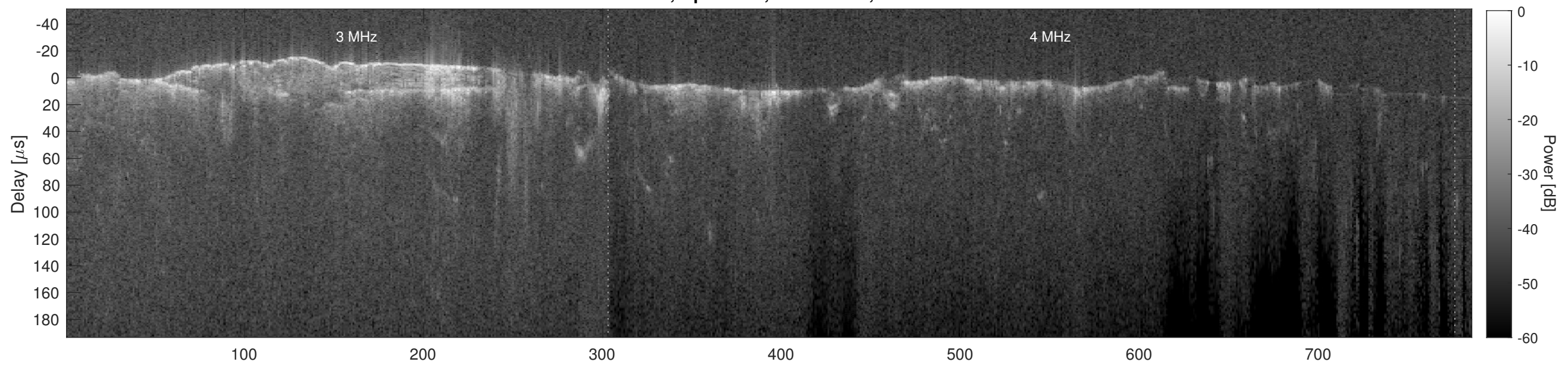
Orbit 14791, Cluttergram
