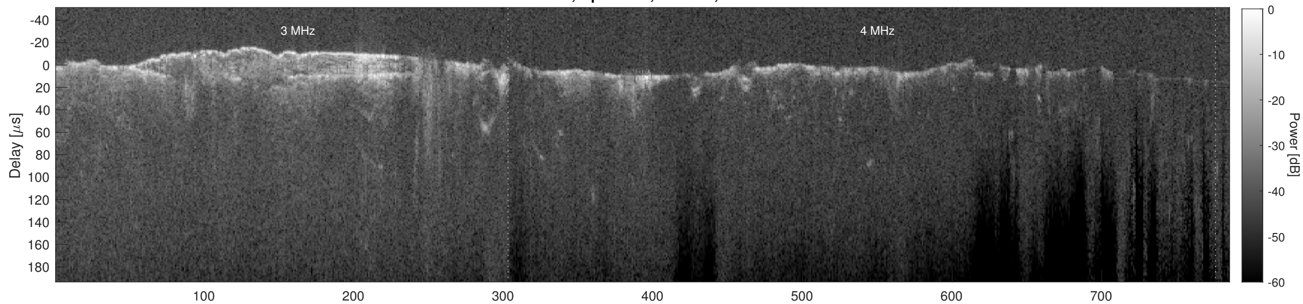
Orbit 14791, Cluttergram
