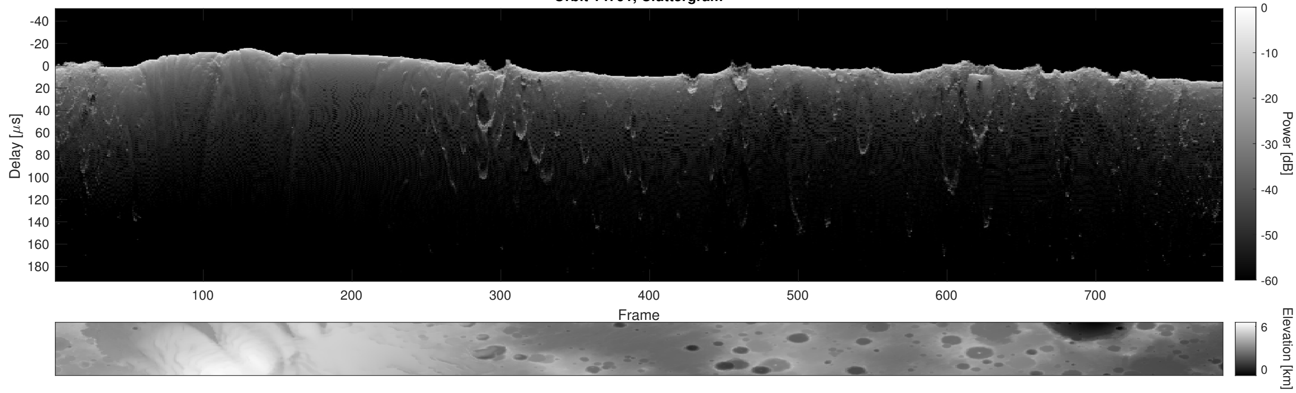
Orbit 14791, Cluttergram
