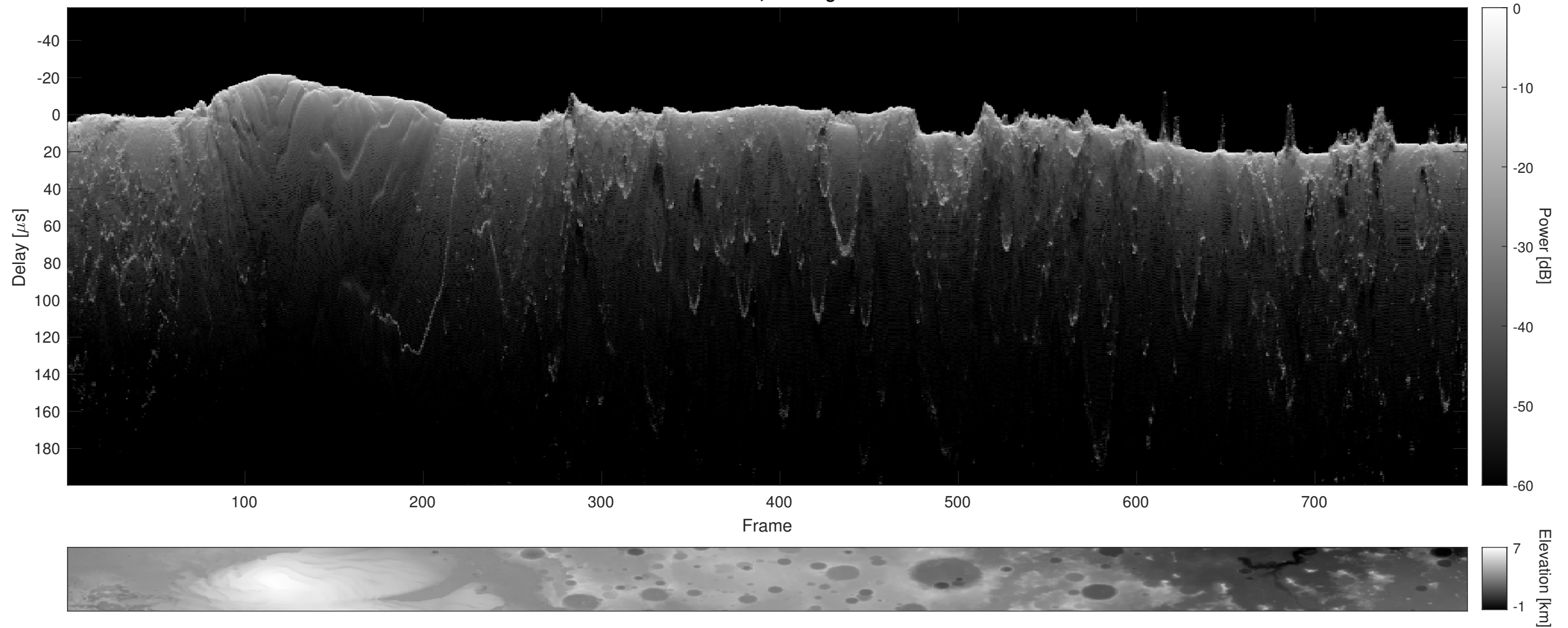
Orbit 14792, Cluttergram
