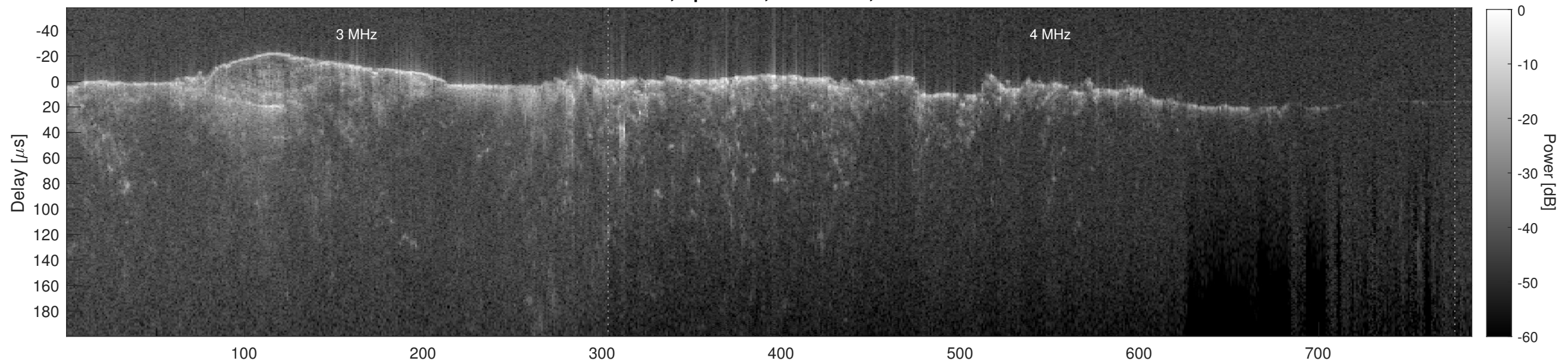
Orbit 14792, Cluttergram
