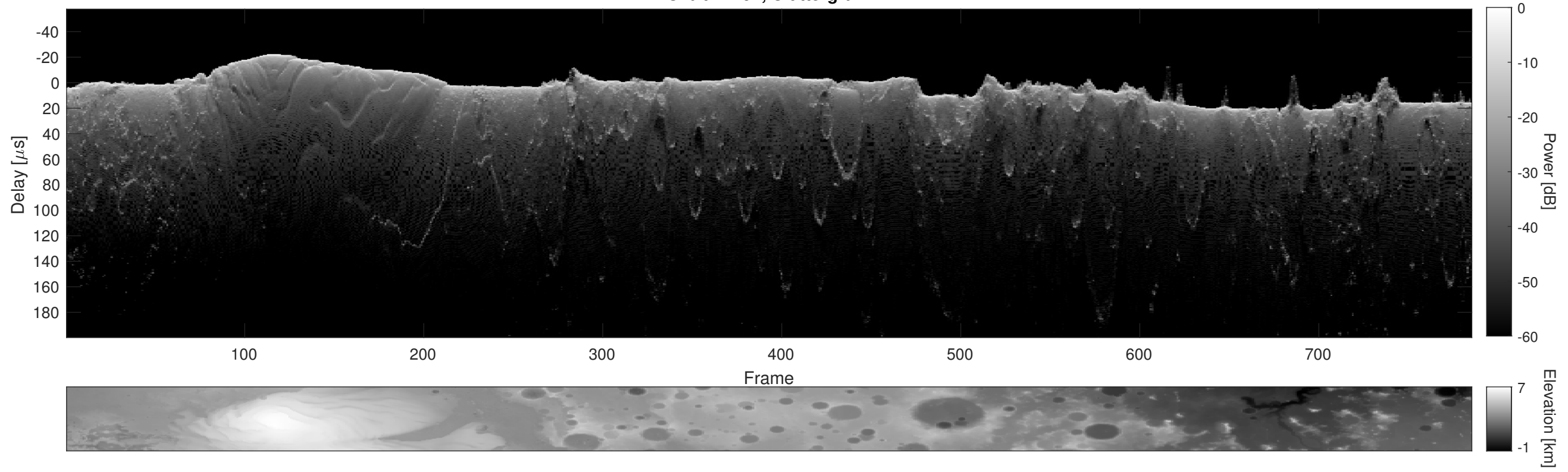
Orbit 14792, Cluttergram
