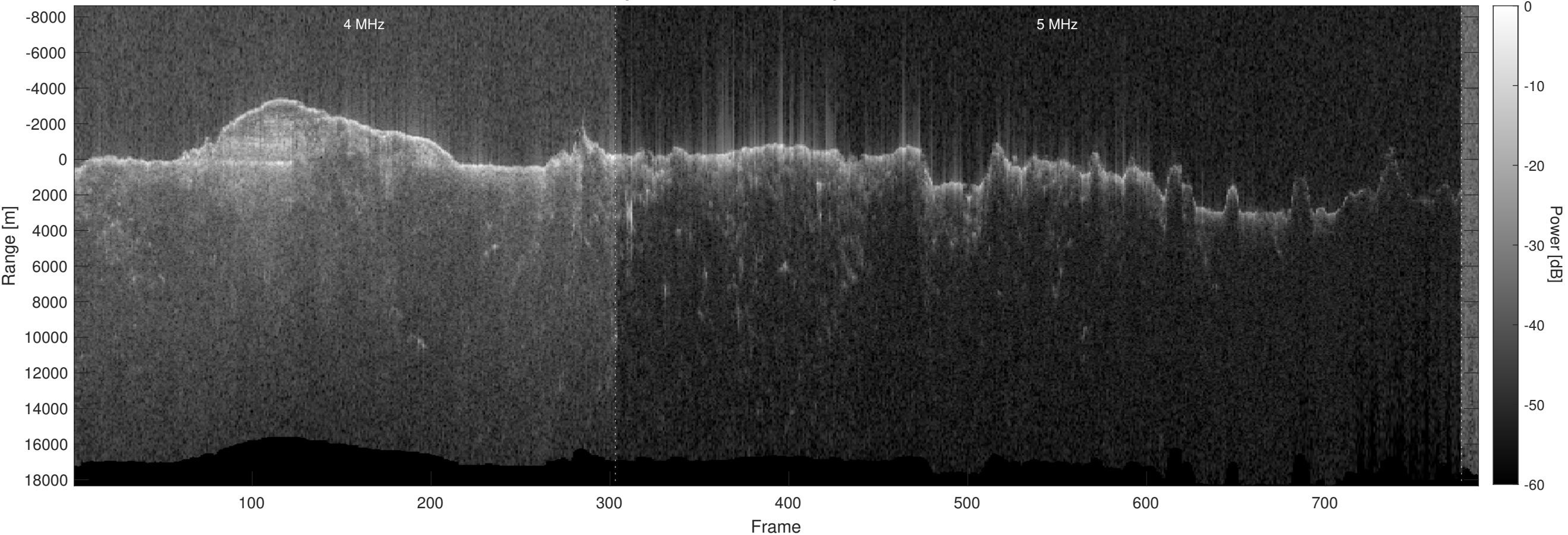
Orbit 14792, Optimized, No Window, Depth-Corrected, Channel 2
