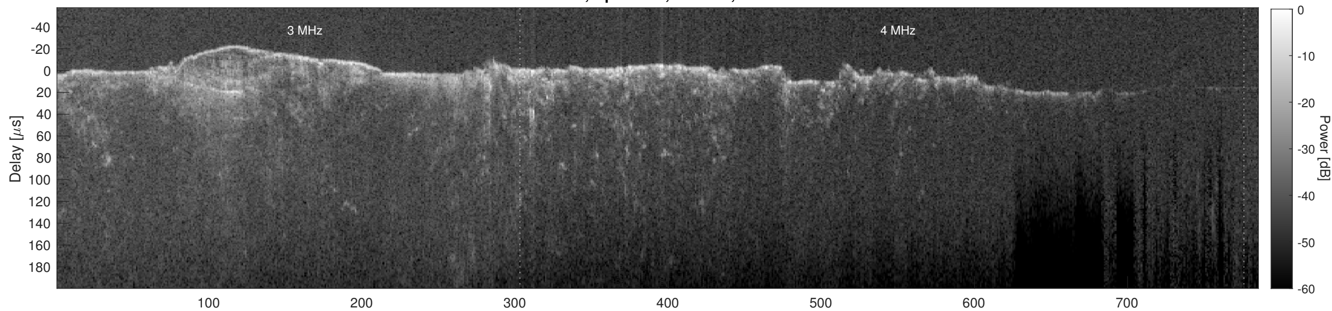
Orbit 14792, Cluttergram
