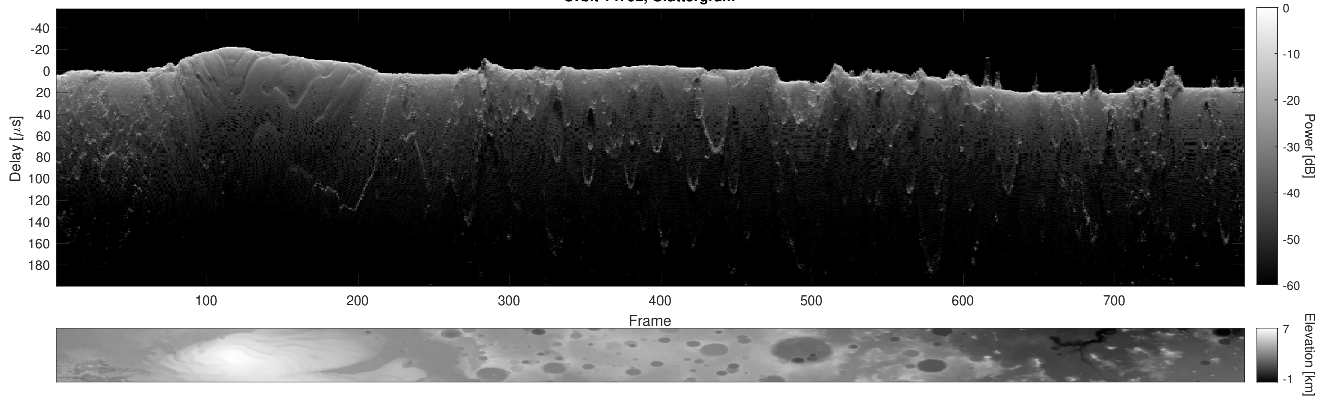
Orbit 14792, Cluttergram
