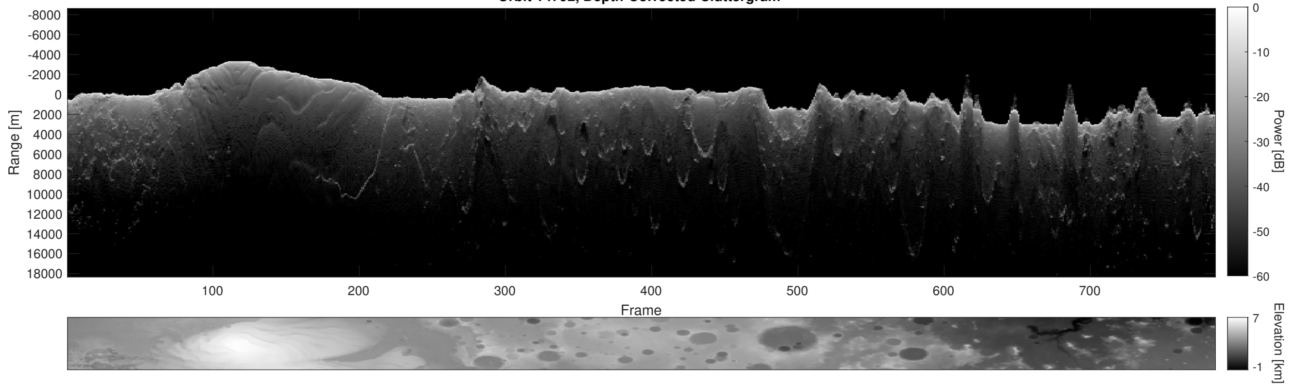
Orbit 14792, Depth-Corrected Cluttergram
