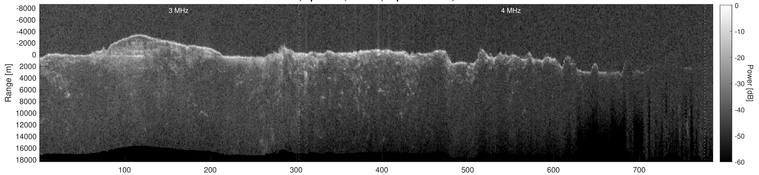
Orbit 14792, Depth-Corrected Cluttergram
