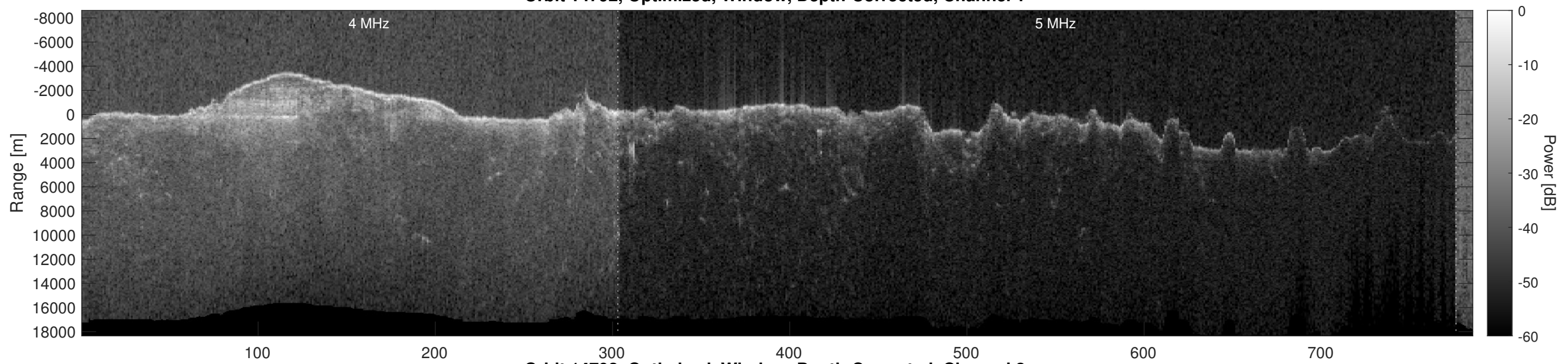
Orbit 14792, Optimized, Window, Depth-Corrected, Channel 2
