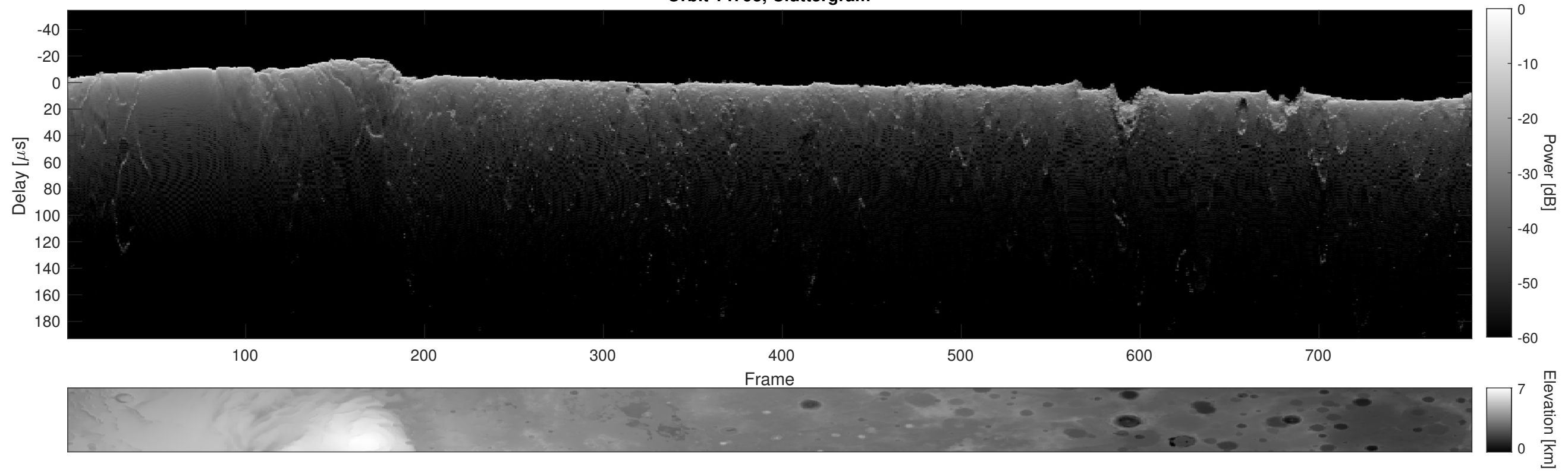
Orbit 14793, Cluttergram
