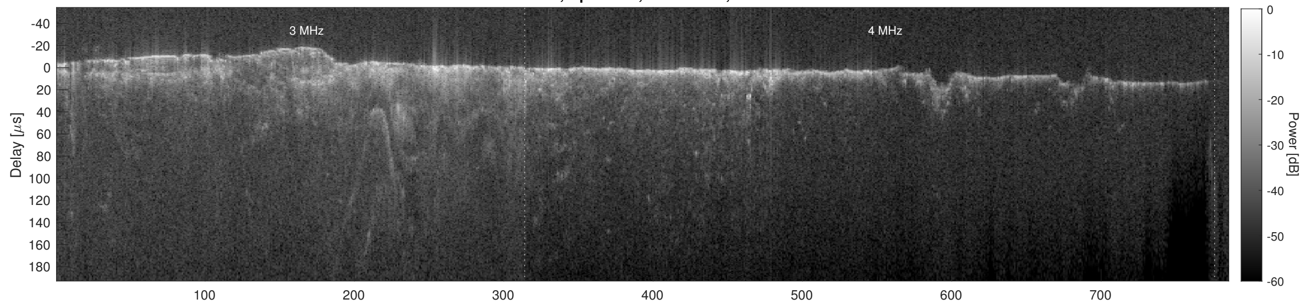
Orbit 14793, Cluttergram
