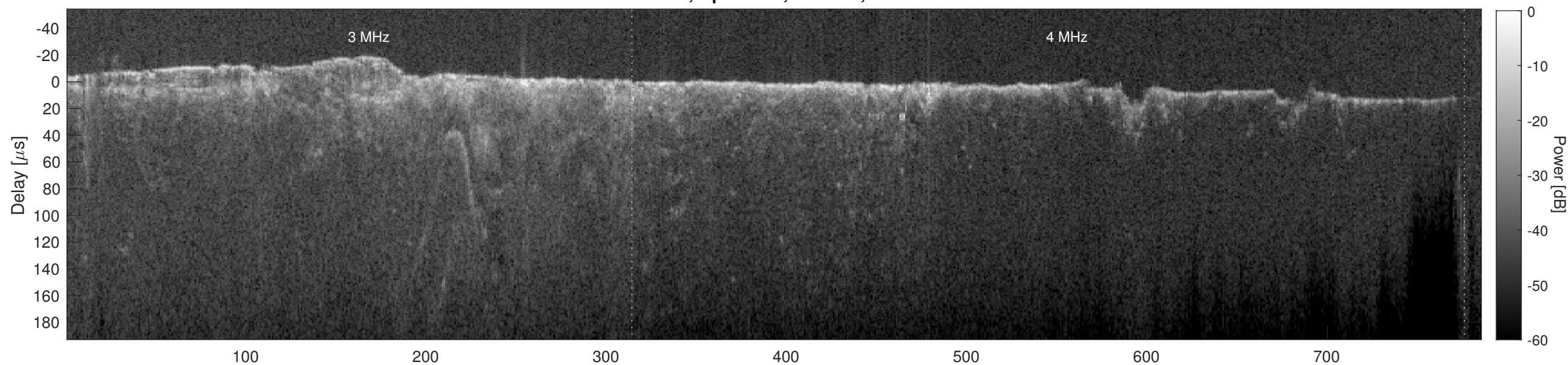
Orbit 14793, Cluttergram
