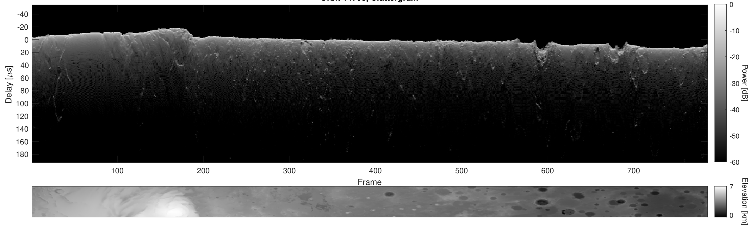
Orbit 14793, Cluttergram
