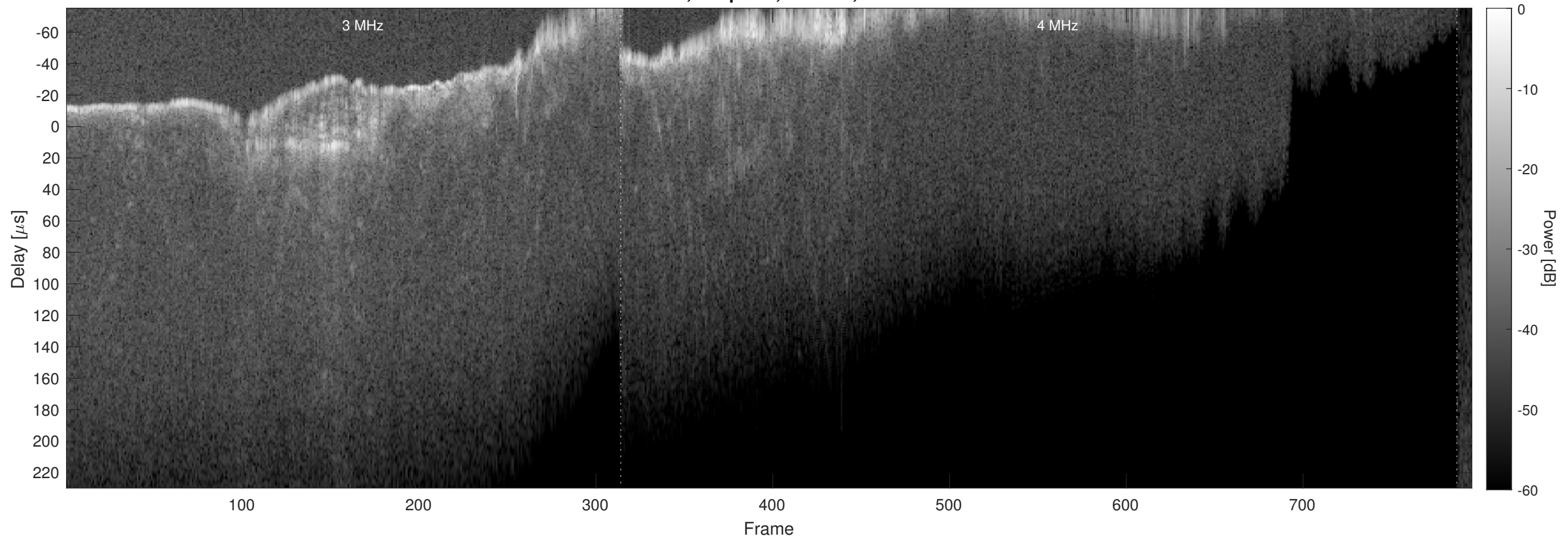
Orbit 14796, Chapman, Window, Channel 2
