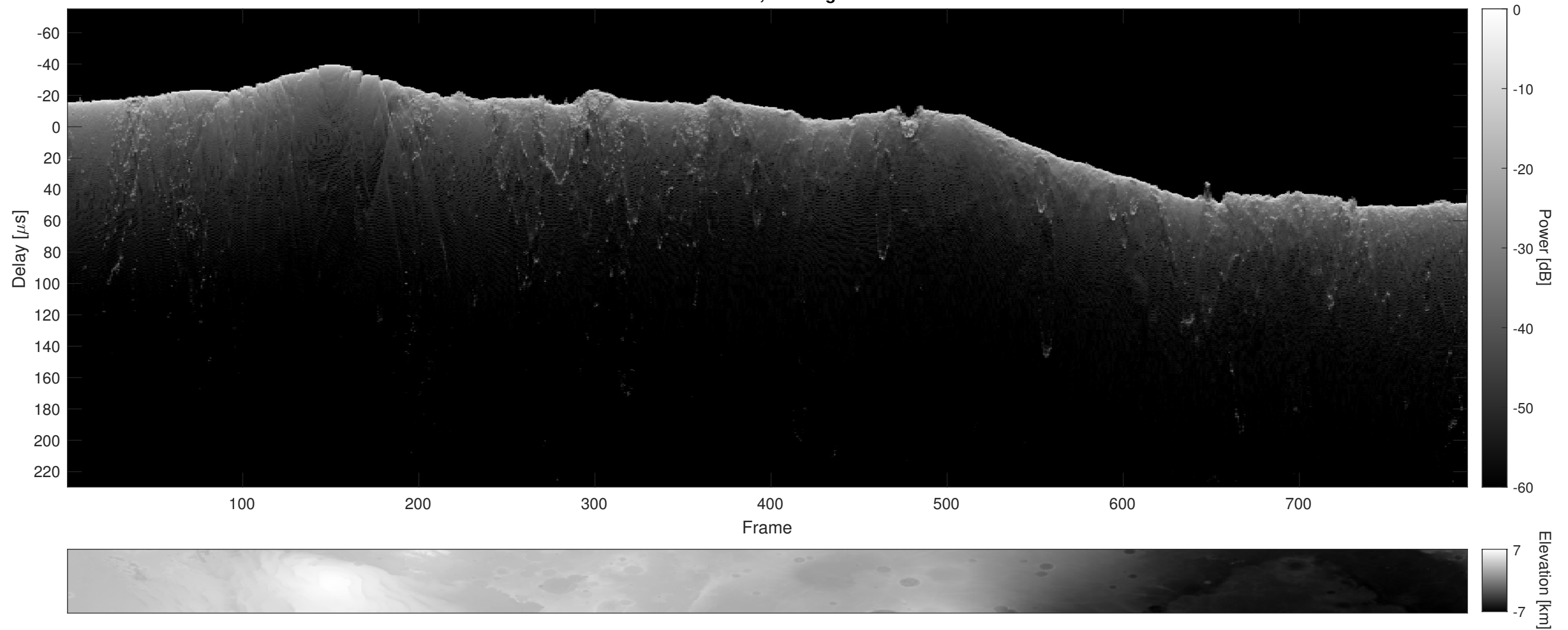
Orbit 14796, Cluttergram
