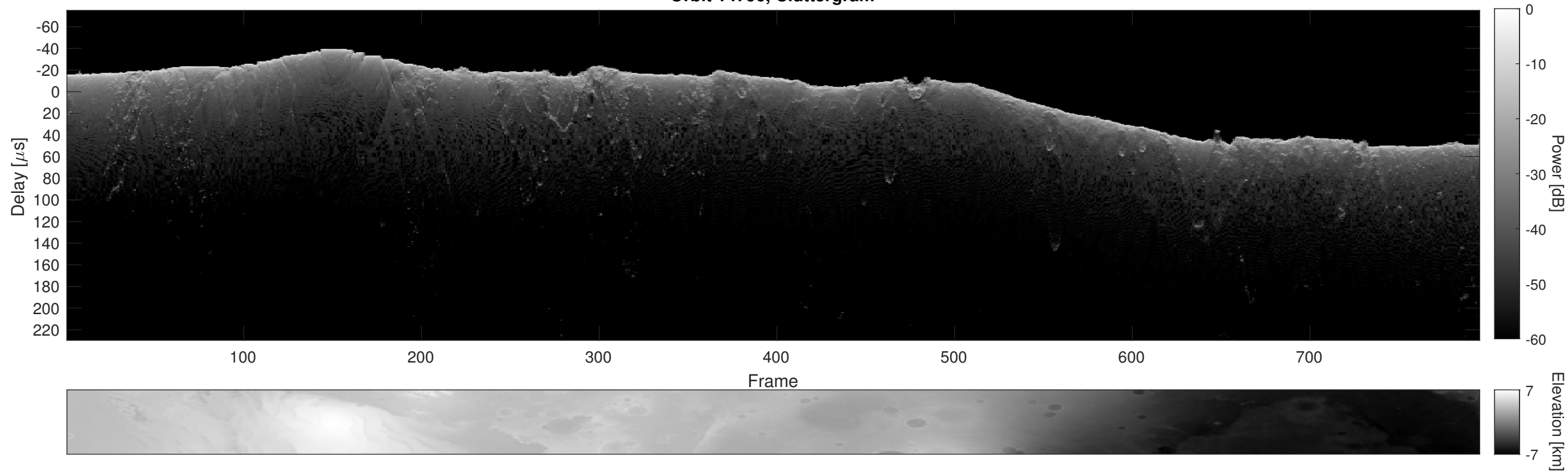
Orbit 14796, Cluttergram
