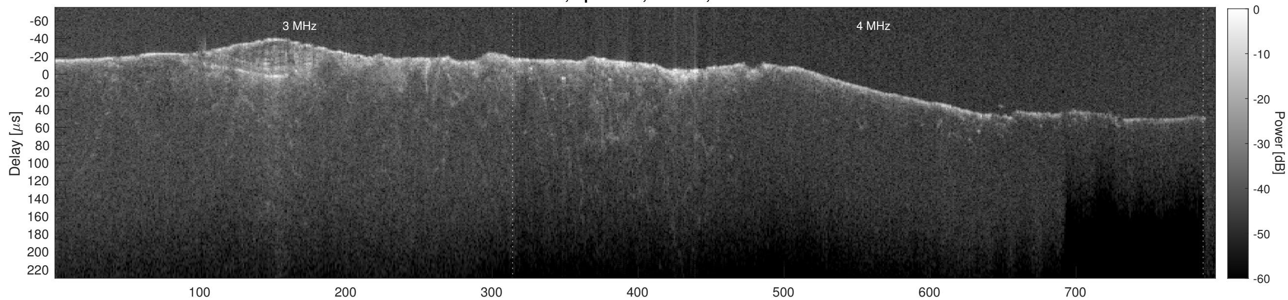
Orbit 14796, Cluttergram
