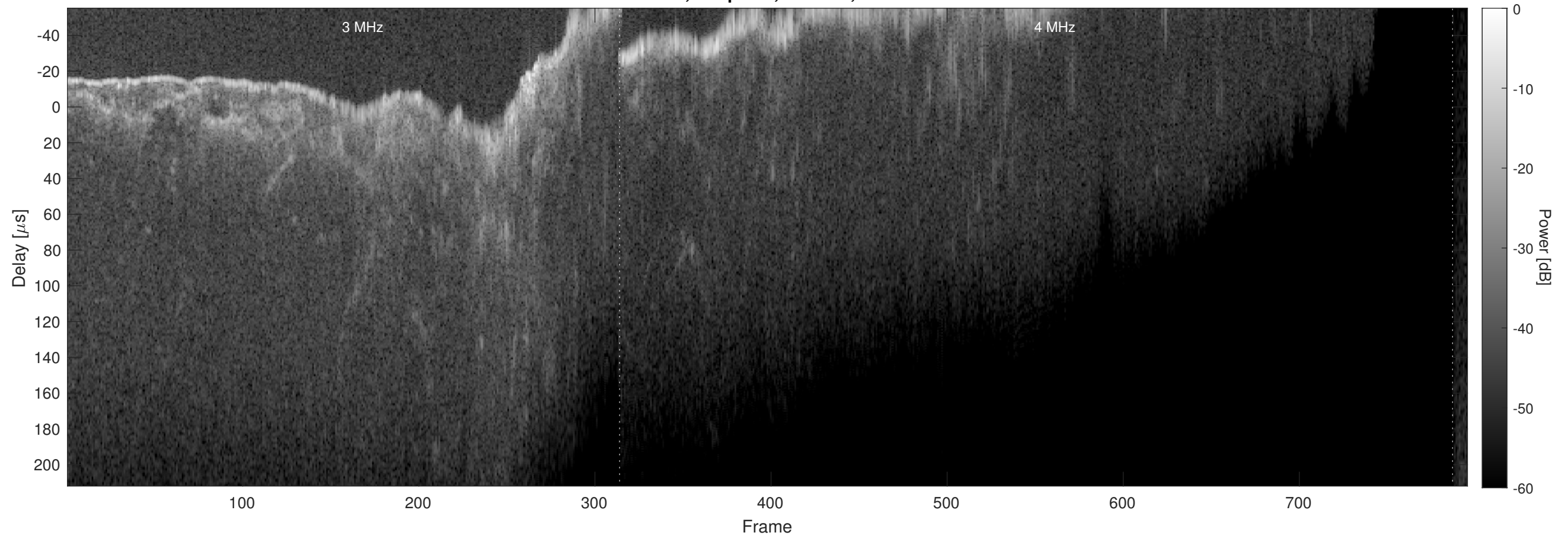
Orbit 14797, Chapman, Window, Channel 2
