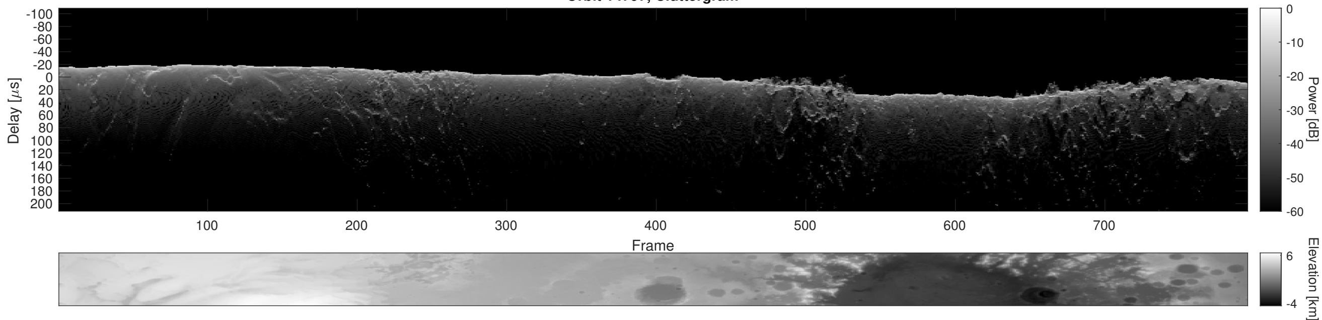
Orbit 14797, Cluttergram
