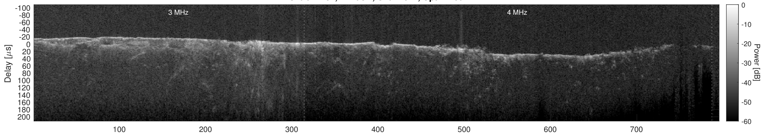
Orbit 14797, Cluttergram
