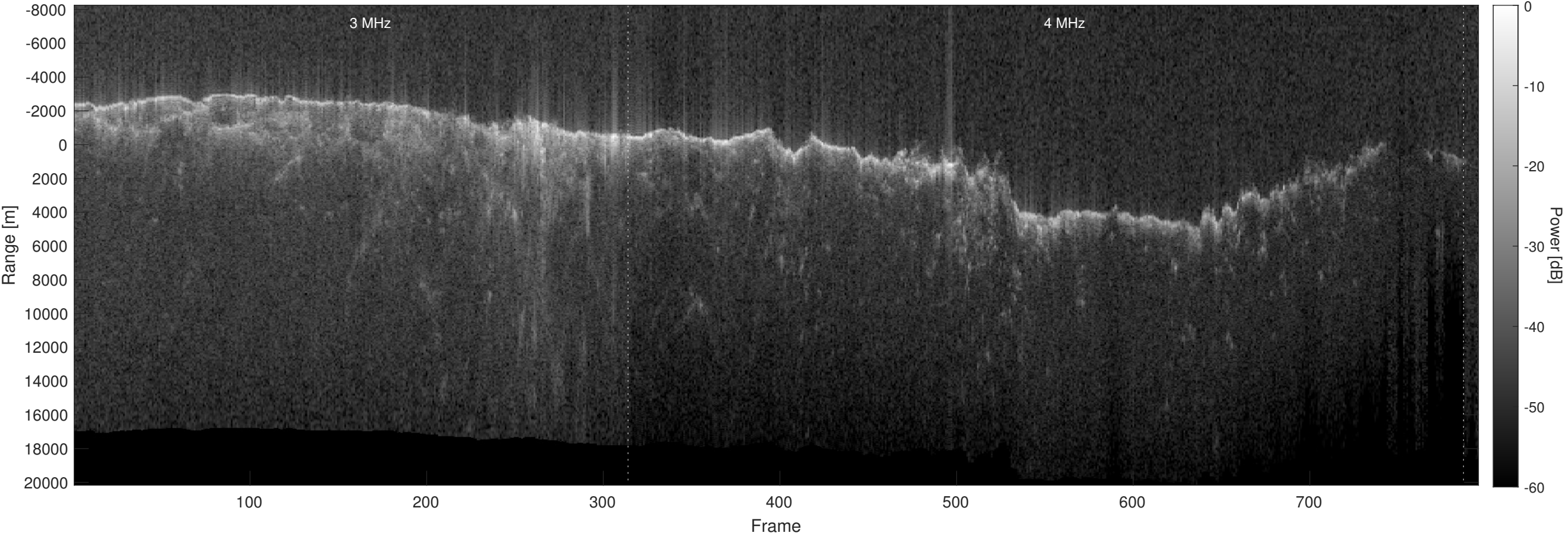
Orbit 14797, Optimized, No Window, Depth-Corrected, Channel 2
