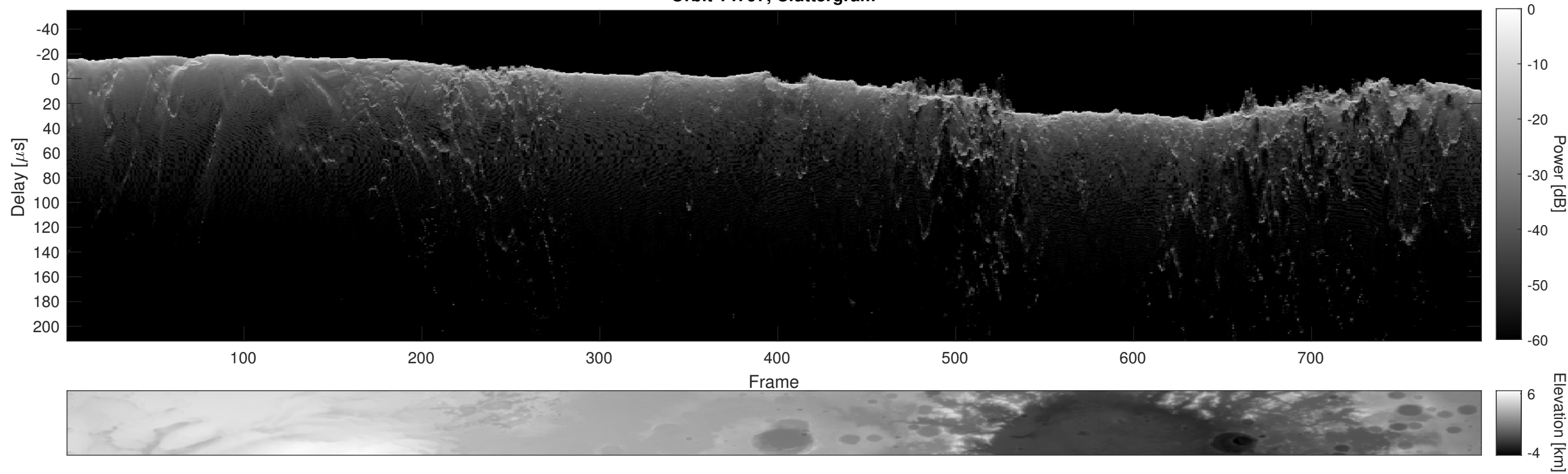
Orbit 14797, Cluttergram
