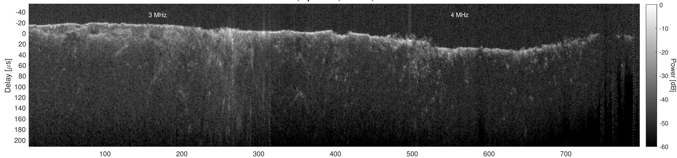
Orbit 14797, Cluttergram
