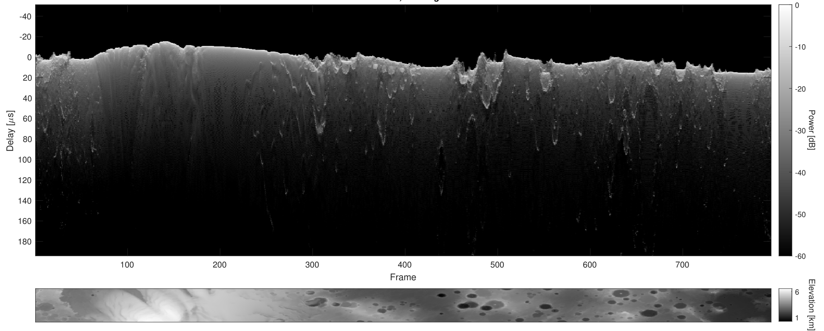
Orbit 14798, Cluttergram
