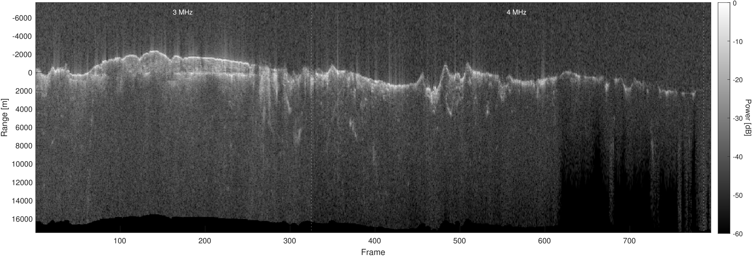
Orbit 14798, Optimized, No Window, Depth-Corrected, Channel 2
