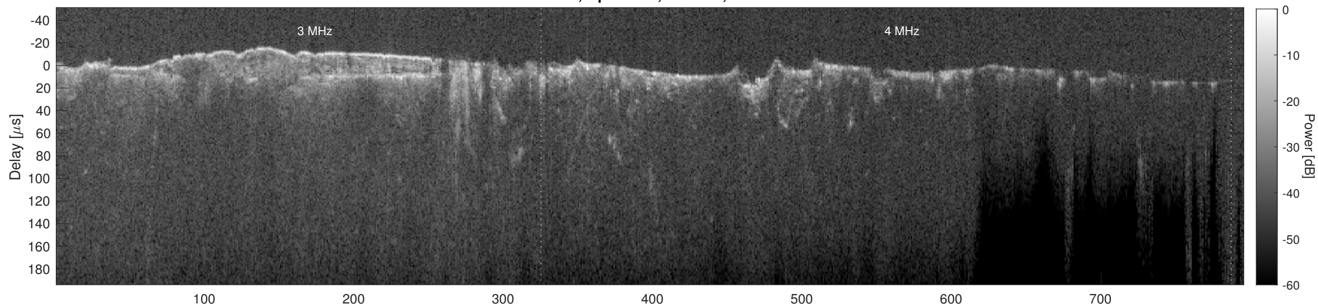
Orbit 14798, Cluttergram
