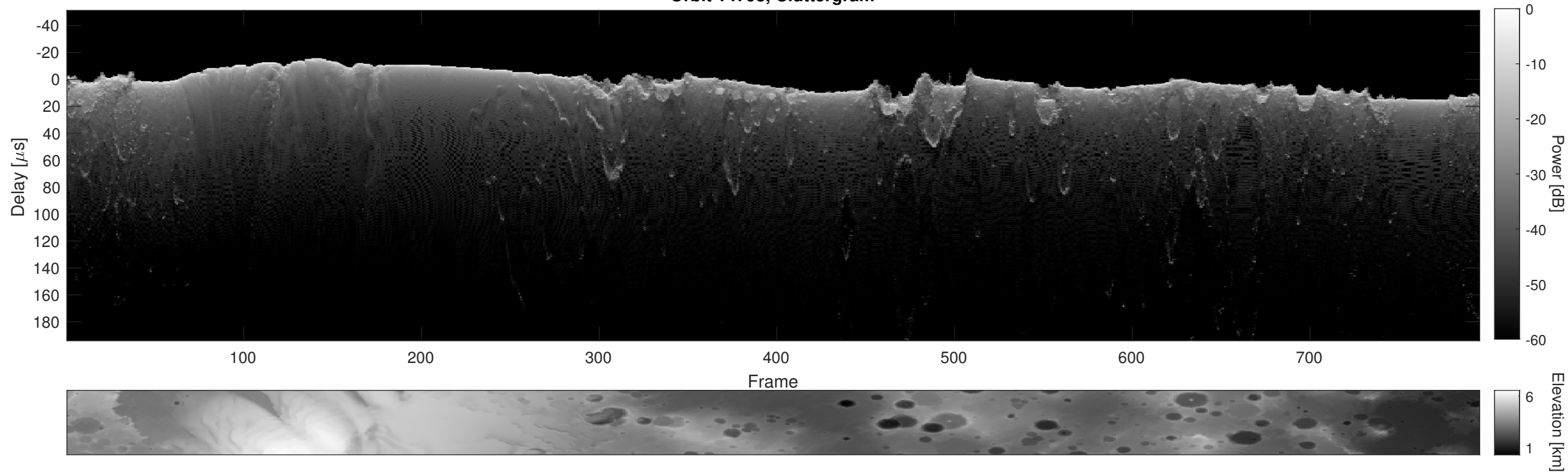
Orbit 14798, Cluttergram
