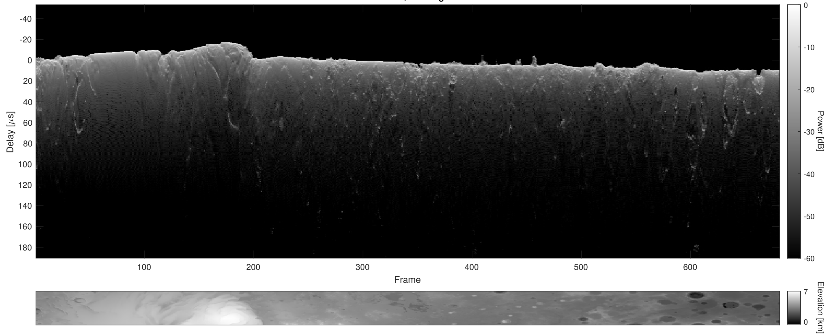
Orbit 14800, Cluttergram
