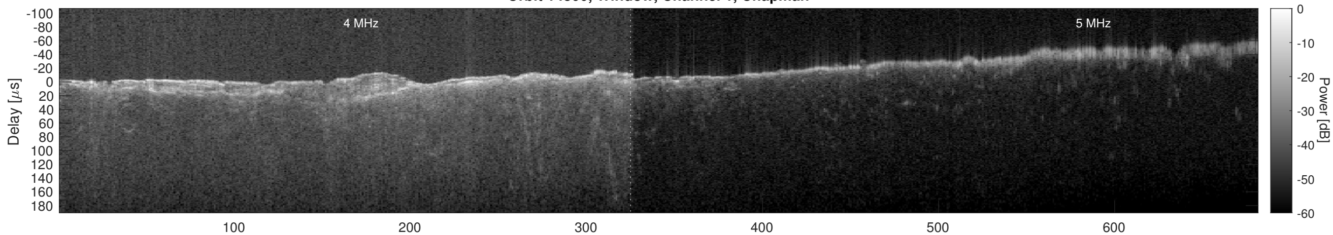
Orbit 14800, Window, Channel 1, Optimized
