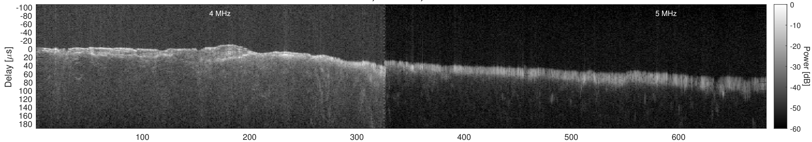
Orbit 14800, Window, Channel 1, Chapman
