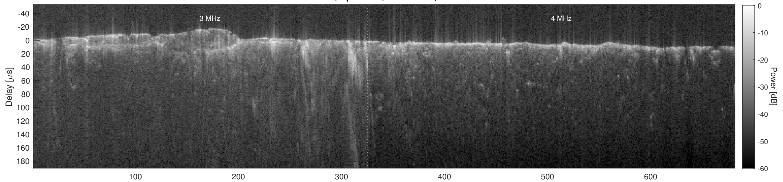
Orbit 14800, Cluttergram
