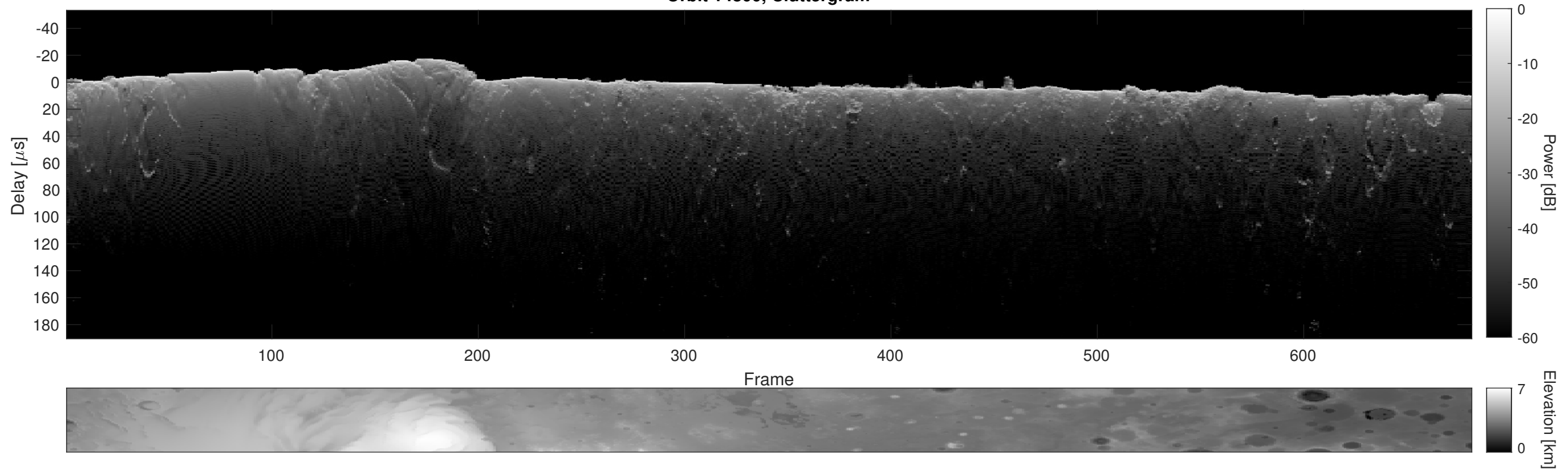
Orbit 14800, Cluttergram
