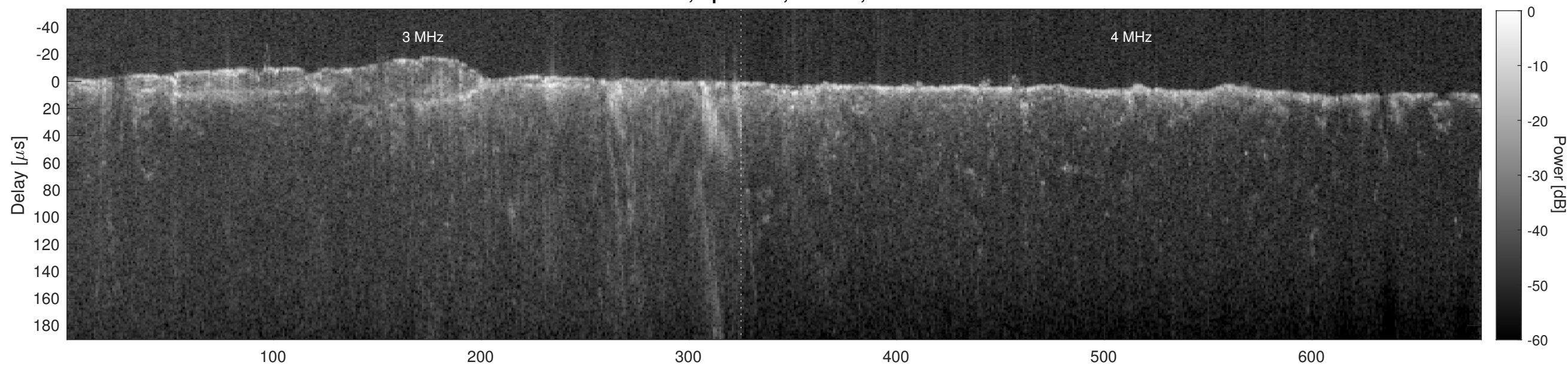
Orbit 14800, Cluttergram
