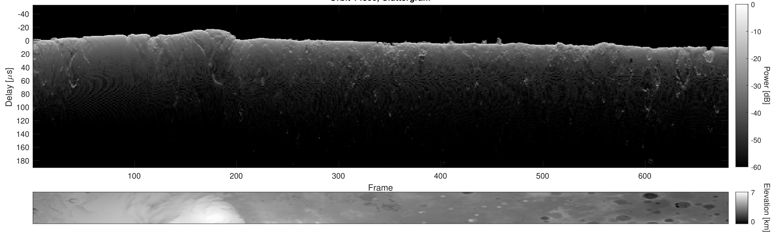
Orbit 14800, Cluttergram
