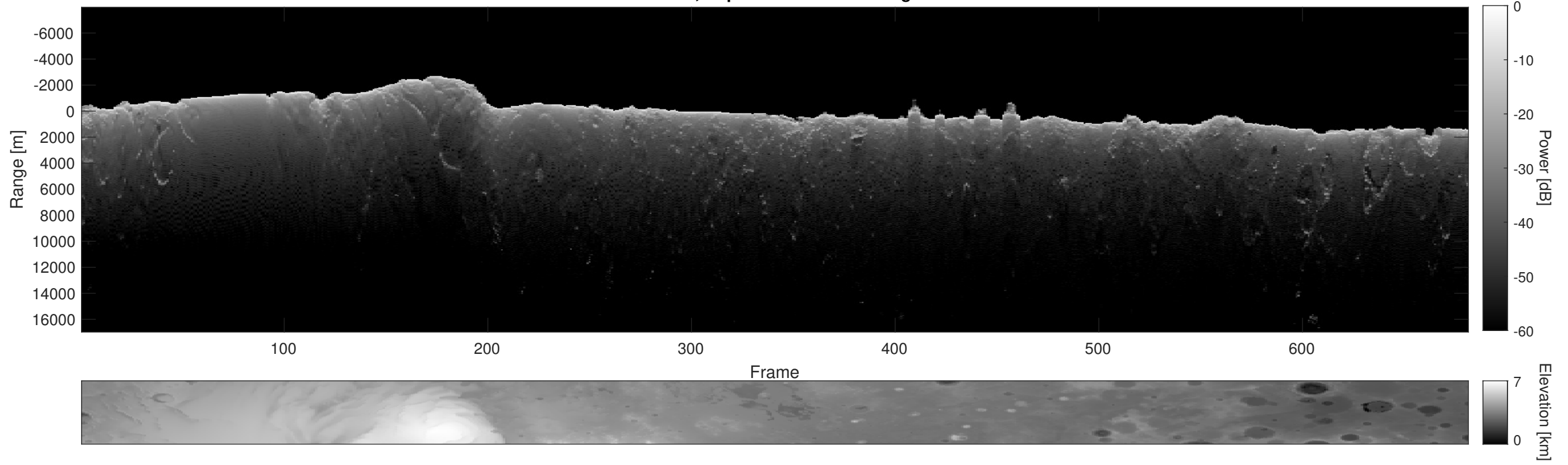
Orbit 14800, Depth-Corrected Cluttergram
