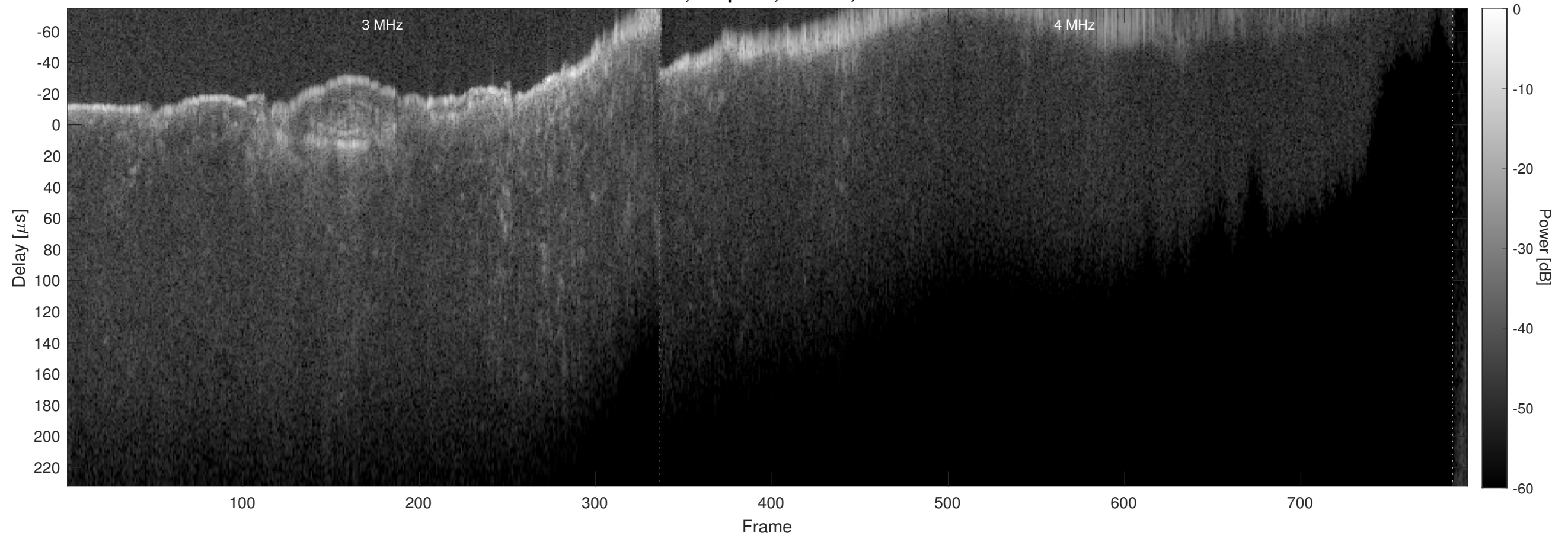
Orbit 14803, Chapman, Window, Channel 2
