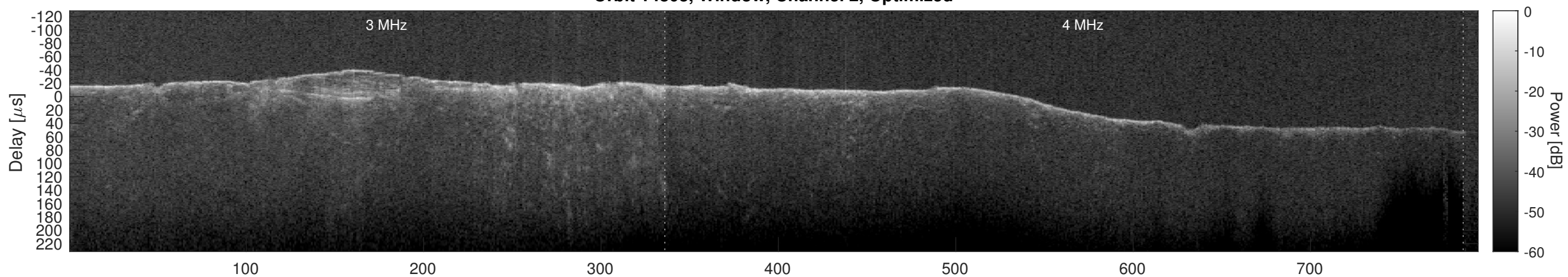
Orbit 14803, Cluttergram
