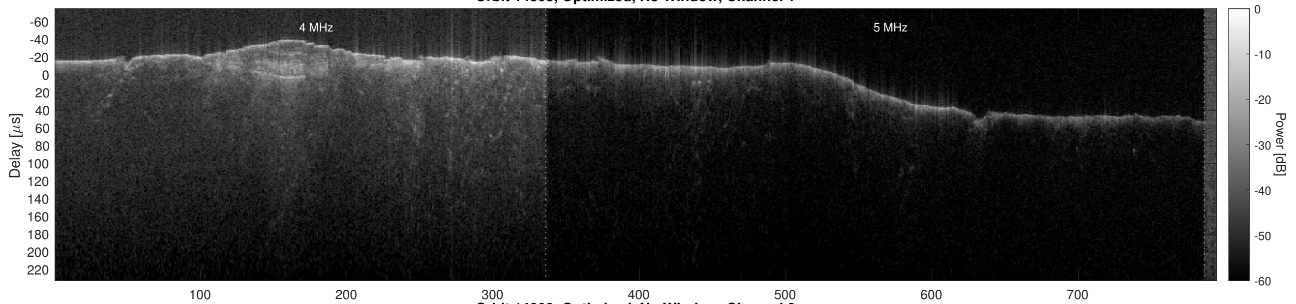
Orbit 14803, Optimized, No Window, Channel 2
