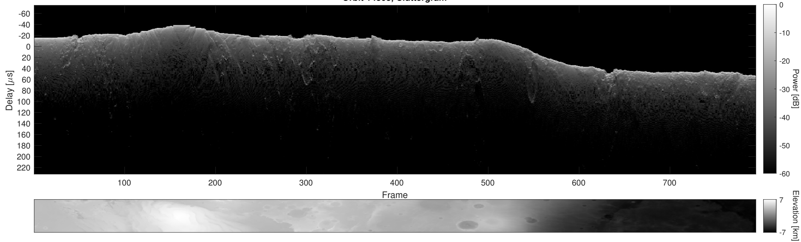
Orbit 14803, Cluttergram
