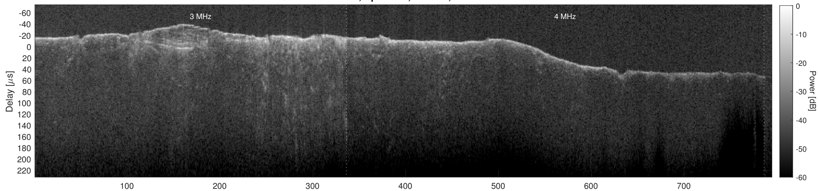
Orbit 14803, Cluttergram
