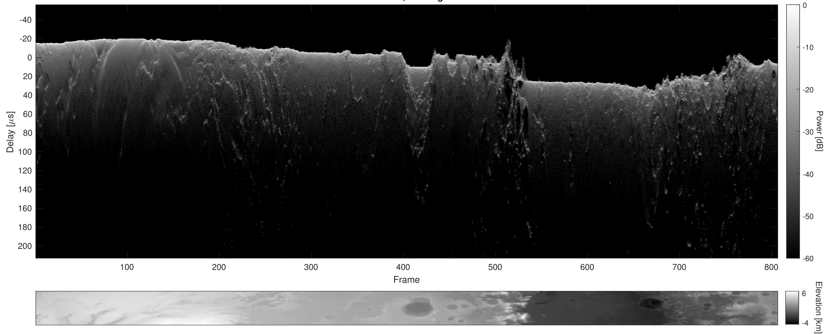
Orbit 14804, Cluttergram
